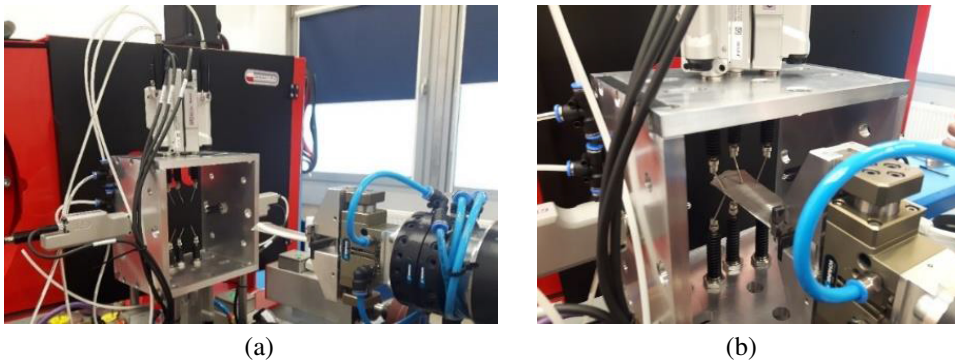
Fig. 15. Pictures of a built measurement module (a), blade geometry measurement in the selected cross-section (b)
