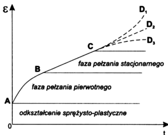
Fig. 3. Phases of rock salt strain (Ślizowski, 2006)
