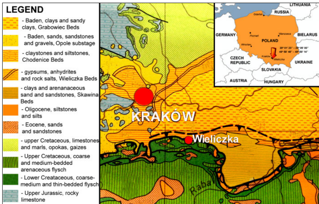
Fig. 1. Fragment of the geological map of Poland without Quaternary formations (based on Rühle, 1977)
