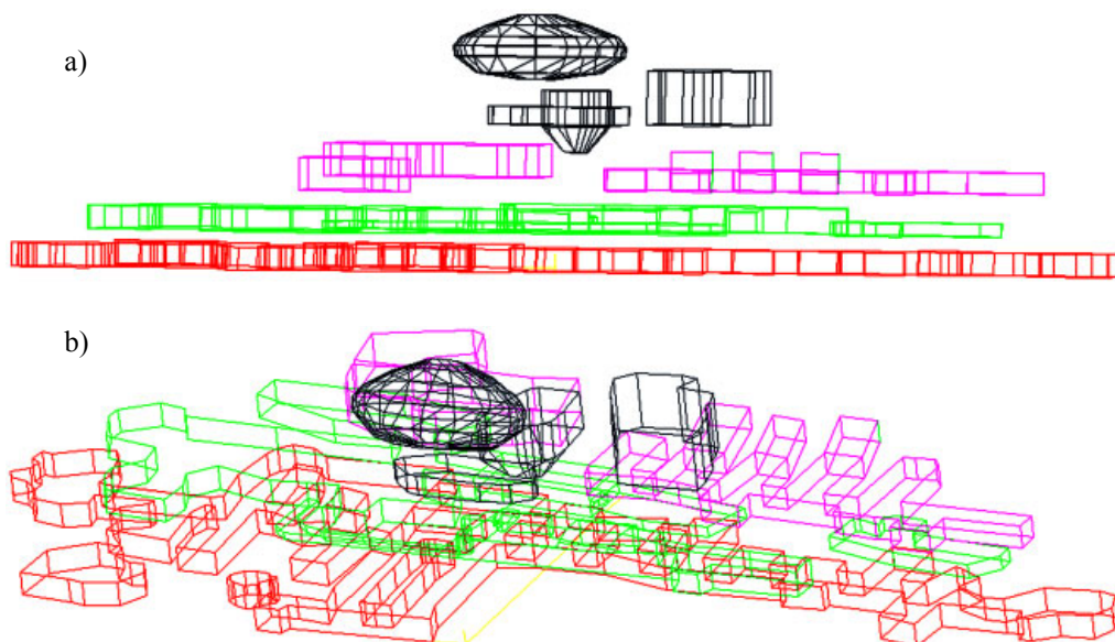
Fig. 4. Summary presentation of the spatial models of chambers in the vicinity of the Warszawa Chamber and Levels from II to III adopted for numerical modelling: a) view from the south on the chamber model, b) view “from the top” towards south-east (Cieřlik et al., 2009)
