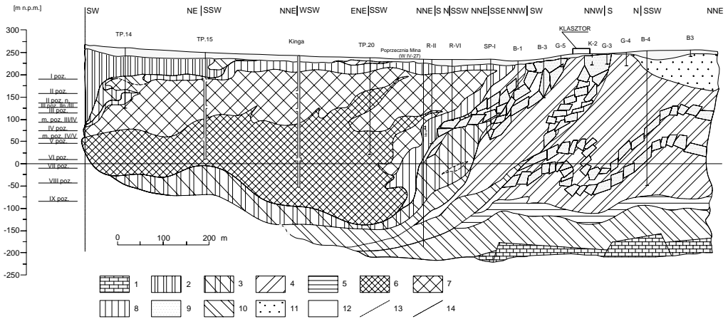
Fig. 2. Geological cross-section of the “Wieliczka” salt bed (Szybist, 2011)
