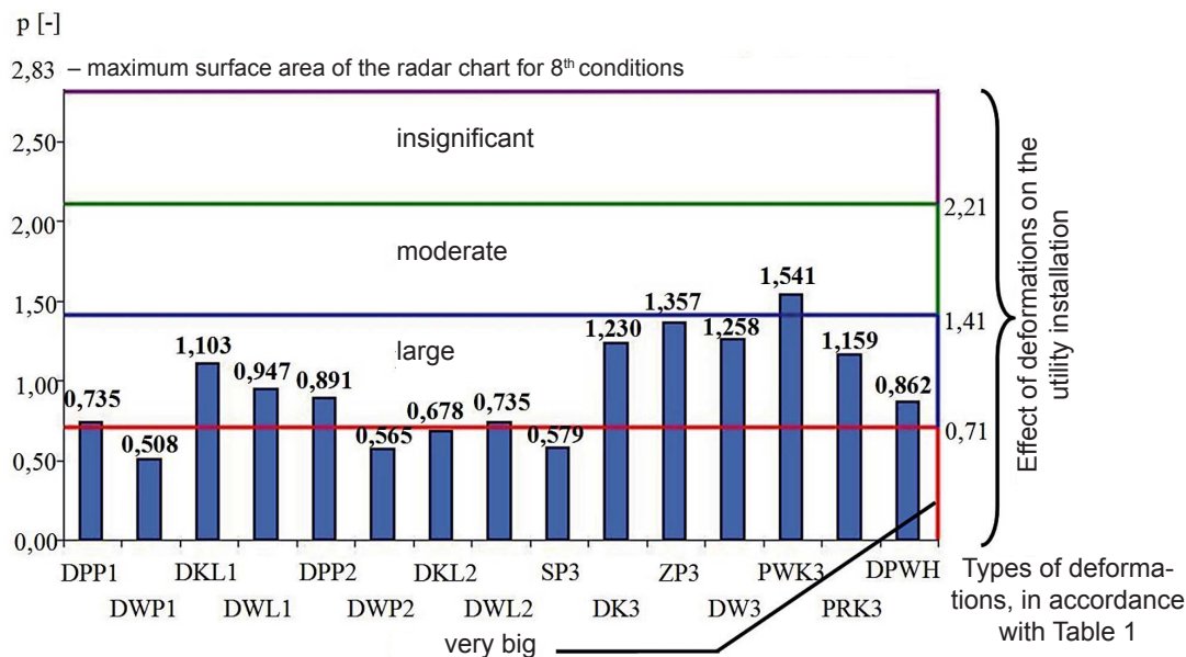
Fig. 4. Set of radar graph areas values describing assembly suitability of assessed welding deformation types of the hybrid node (on the basis of [6])
