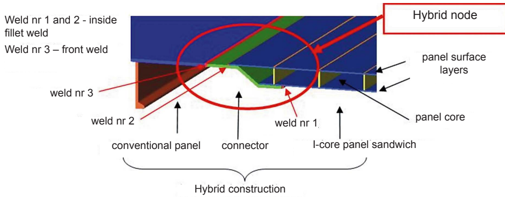
Fig. 1. Hybrid node [6, 8]
