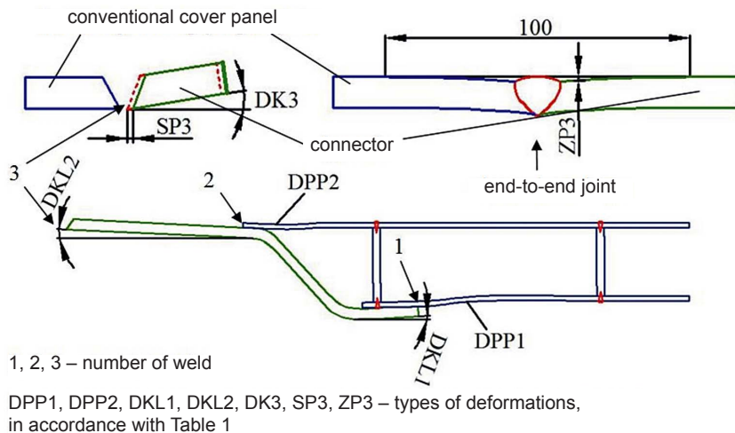
Fig. 2. Selected types of welding deformations distinguished in the hybrid node [6, 7]
