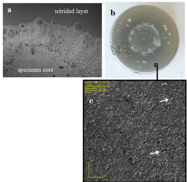
Fig. 8. Corroded surface morphology of plasma nitrided in 35:65 H 2 :N 2 working gas mixture 440B steel; a – SEM photograph, magnification 50×; b – macro photograph; c – confocal microscope photograph in 1080× magnification, arrows – transition phase particles
