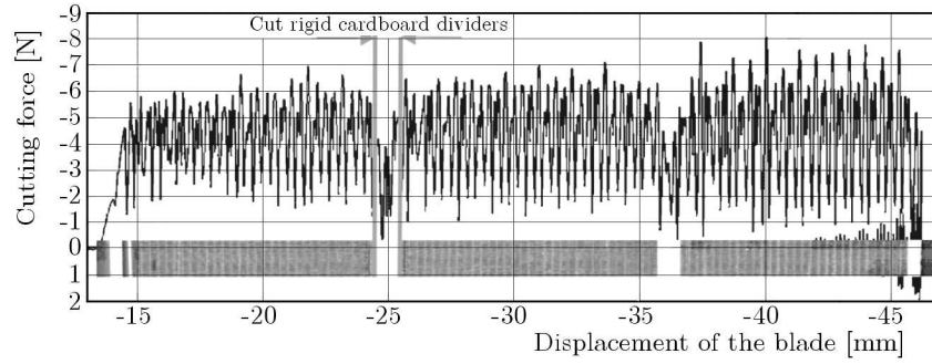
Fig. 10. Dependence between the cutting force and the blade displacement
