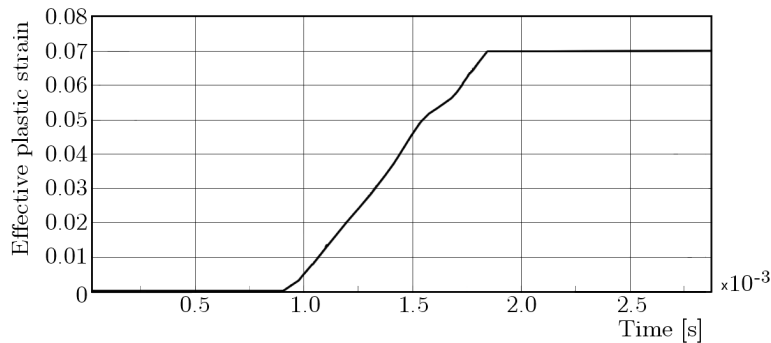
Fig. 6. Characteristics of the plasticization process for a selected SPH particle describing the aluminum plate in the cutting area, up to the moment of decohesion (particle deactivation)
