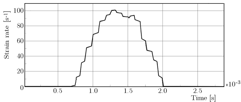
Fig. 7. Diagram of the deformation speed for a selected SPH particle describing the aluminum plate in the cutting area, up to the moment of decohesion (particle deactivation)
