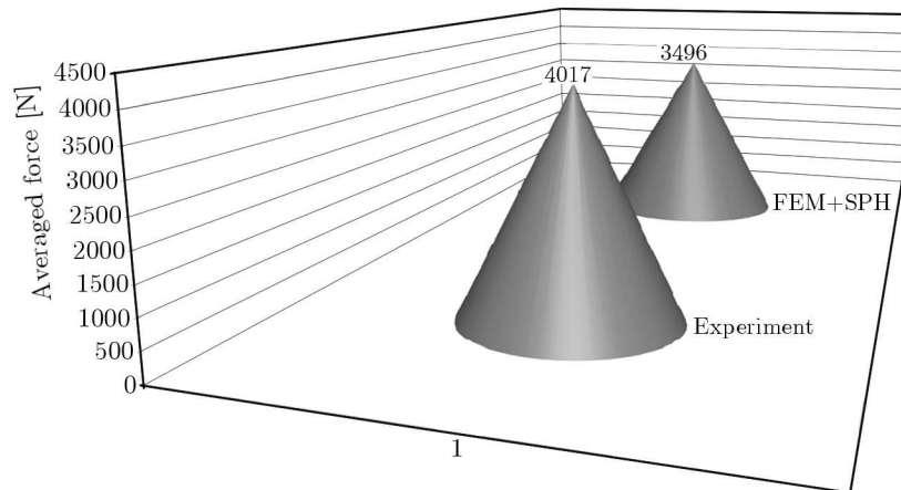
Fig. 12. Characteristics of the force measured in the indicated point – comparison of the results
