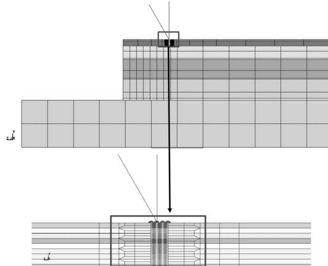
Fig. 2. FEM + SPH coupled model for the performance of numerical tests of the aluminum sheets cutting process
