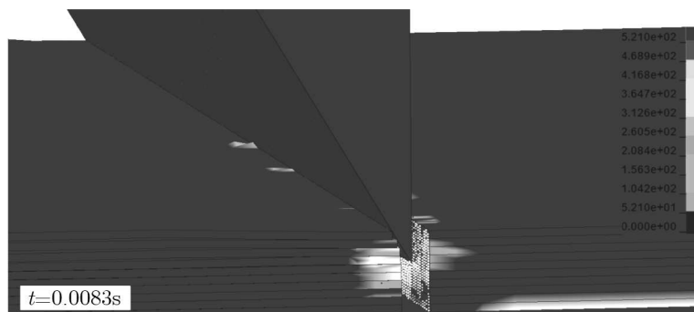
Fig. 4. Reduced stress according to H-M-H in the contact area of the guillotine blade and the layers of the cut aluminum plate in consecutive moments of time
