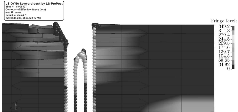
Fig. 5. Behavior of the separated particles of the cut material in the SPH method
