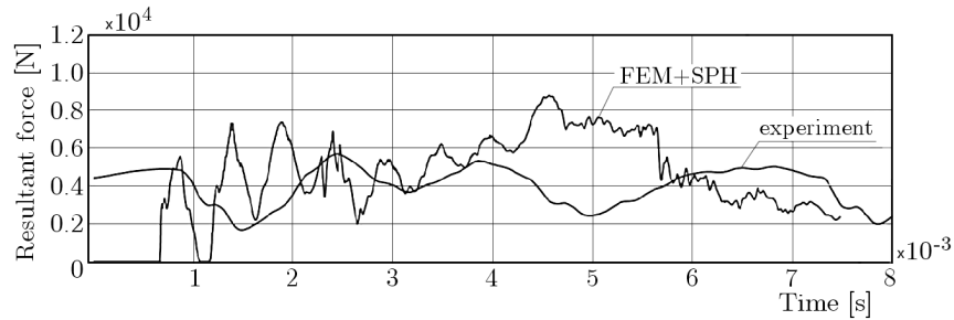
Fig. 11. A comparison of the resultant force of the experiment and the FEM + SPH method
