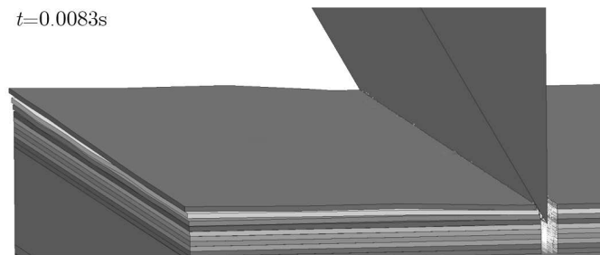
Fig. 3. Deformation of sheet metal obtained in the process of numerical cutting for the FEM + SPH model in selected moments of time
