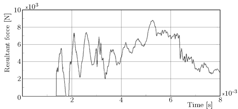
Fig. 9. Characteristics of the force measured in the indicated point, resulting from the sheet metal cutting process for the FEM + SPH model
