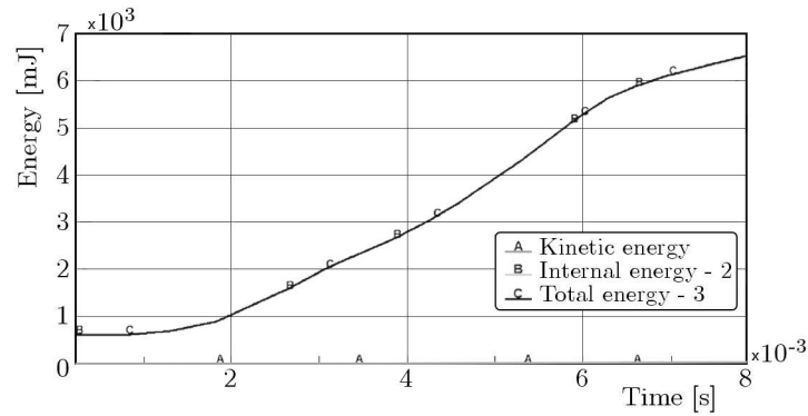
Fig. 8. Energy balance characteristics [ 10^{-6} kJ]
