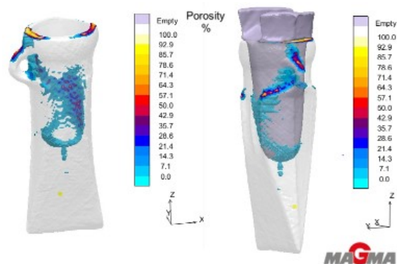
Fig. 3. Simulation of casting porosity when using double-channel main runner [5]
