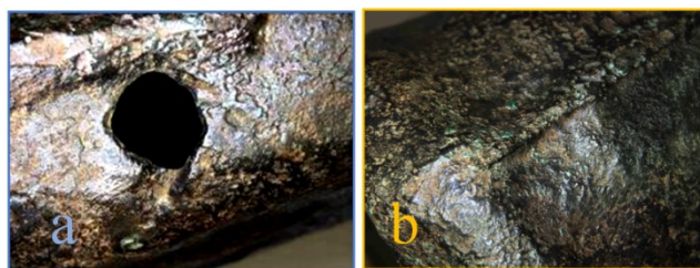
Fig. 7. Axe (No. NG26) with casting defects: incomplete filling - misrun (a) and flashes along the line joining the mould – casting seam (b)
