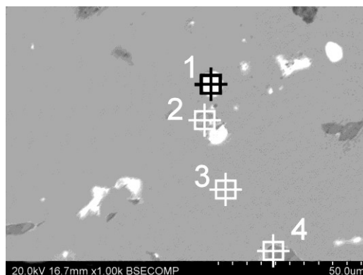
Fig. 12. The SEM images of the axle (NG21) microstructure with the EDS micro-areas spots (refer to table 2)
