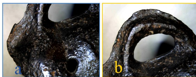
Fig. 6. Axe (No. NG7) with remained elements of the gating system and casting defects: incomplete filling - misrun (a) and flashes along the line joining the mould (b)
