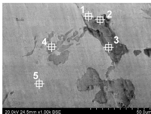
Fig. 13. The SEM images of the axle (NG26) microstructure with the EDS micro-areas spots (refer to table 3)
