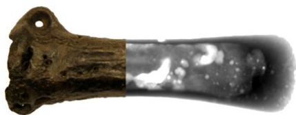
Fig. 8. X-ray image of axe No. NG24 together with the view of part of the artefact with visible defects
