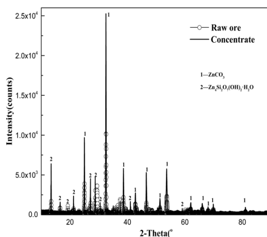
Fig. 10. XRD results of zinc oxide raw ore and its concentrate, raw ore - \text{ZnCO}_3 , \text{Zn}_4\text{Si}_2\text{O}_7(\text{OH})_2 \cdot \text{H}_2\text{O} , \text{MgCO}_3 , \text{CaCO}_3 ; concentrate - \text{ZnCO}_3 , \text{Zn}_4\text{Si}_2\text{O}_7(\text{OH})_2 \cdot \text{H}_2\text{O}
