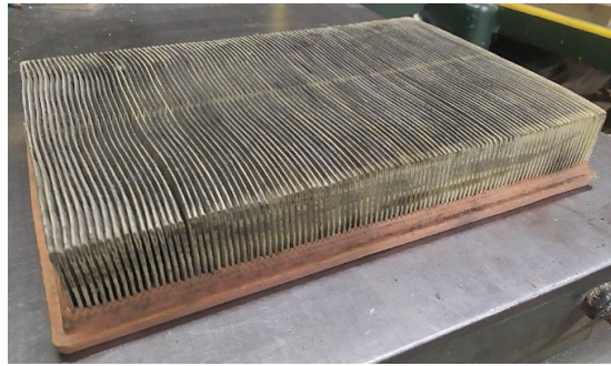
Fig. 11. Used standard air filter with a mileage of 20,000 km
