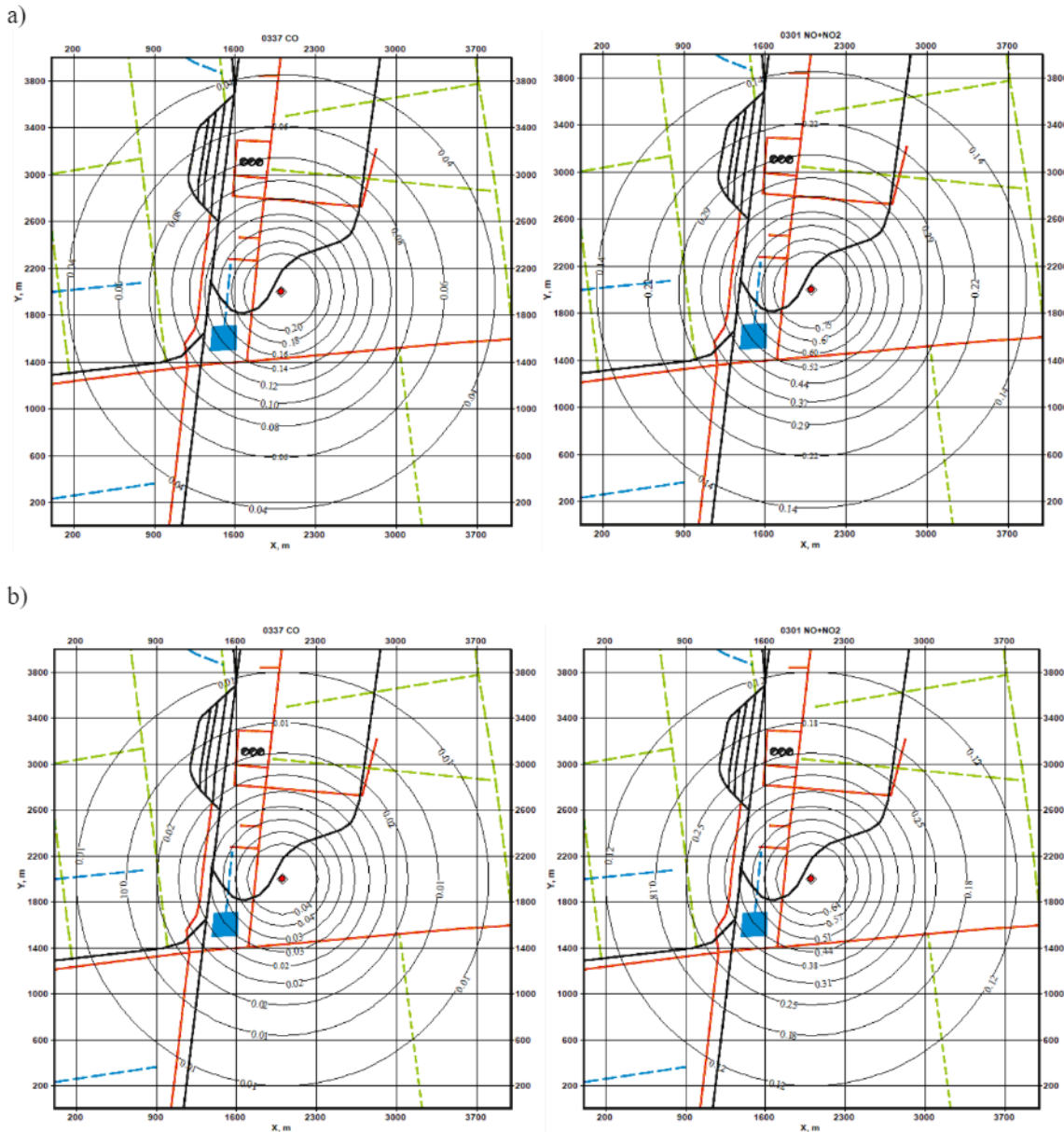
Fig. 2. Fields of ground-level concentrations of hazardous substances around the SAS in 2008 (a) and 2020 (b)
