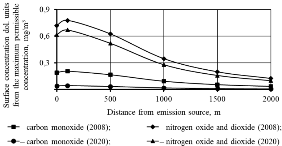
Fig. 3. Dependences of ground-level concentrations of hazardous substances with increasing distance from SAS
