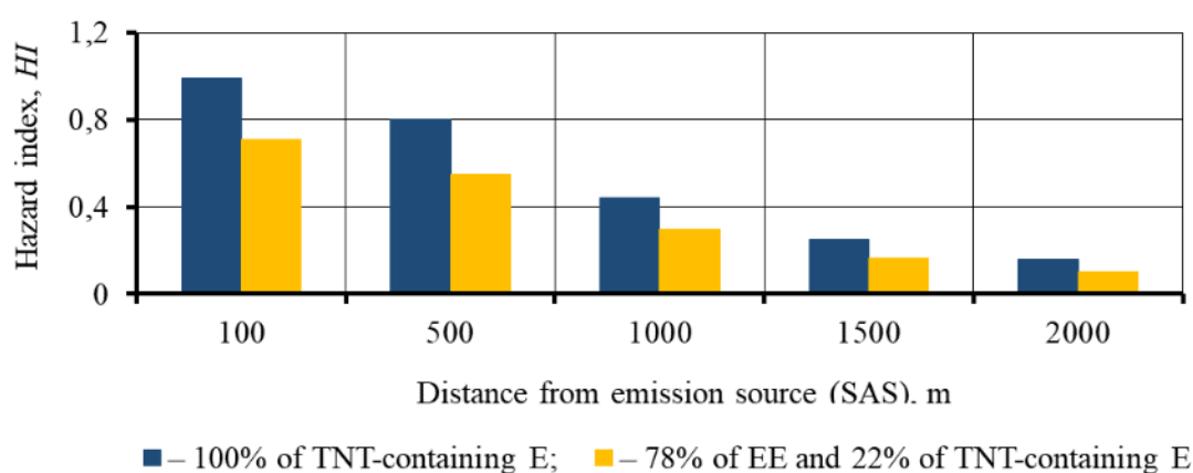
Fig. 4. The nature of the change in the hazard index depending on the distance to the release source
