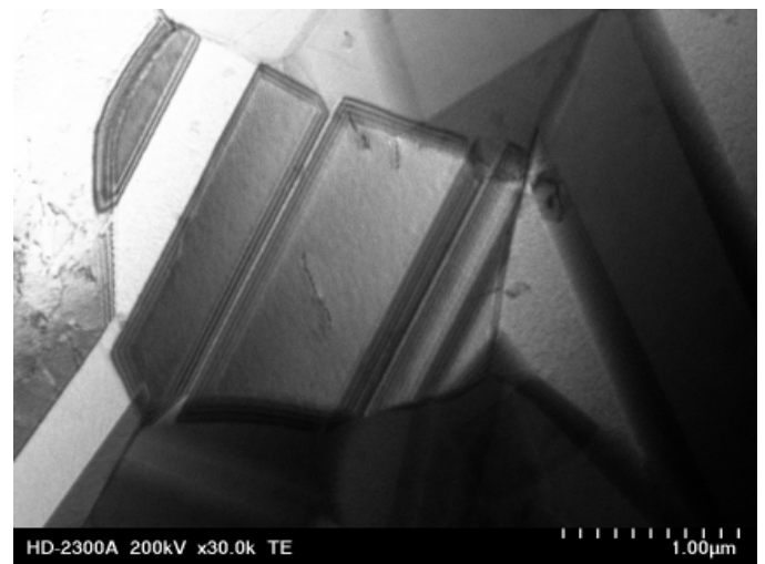
Fig. 11. Microstructure of CuSn20 alloy after KOB, TEM
