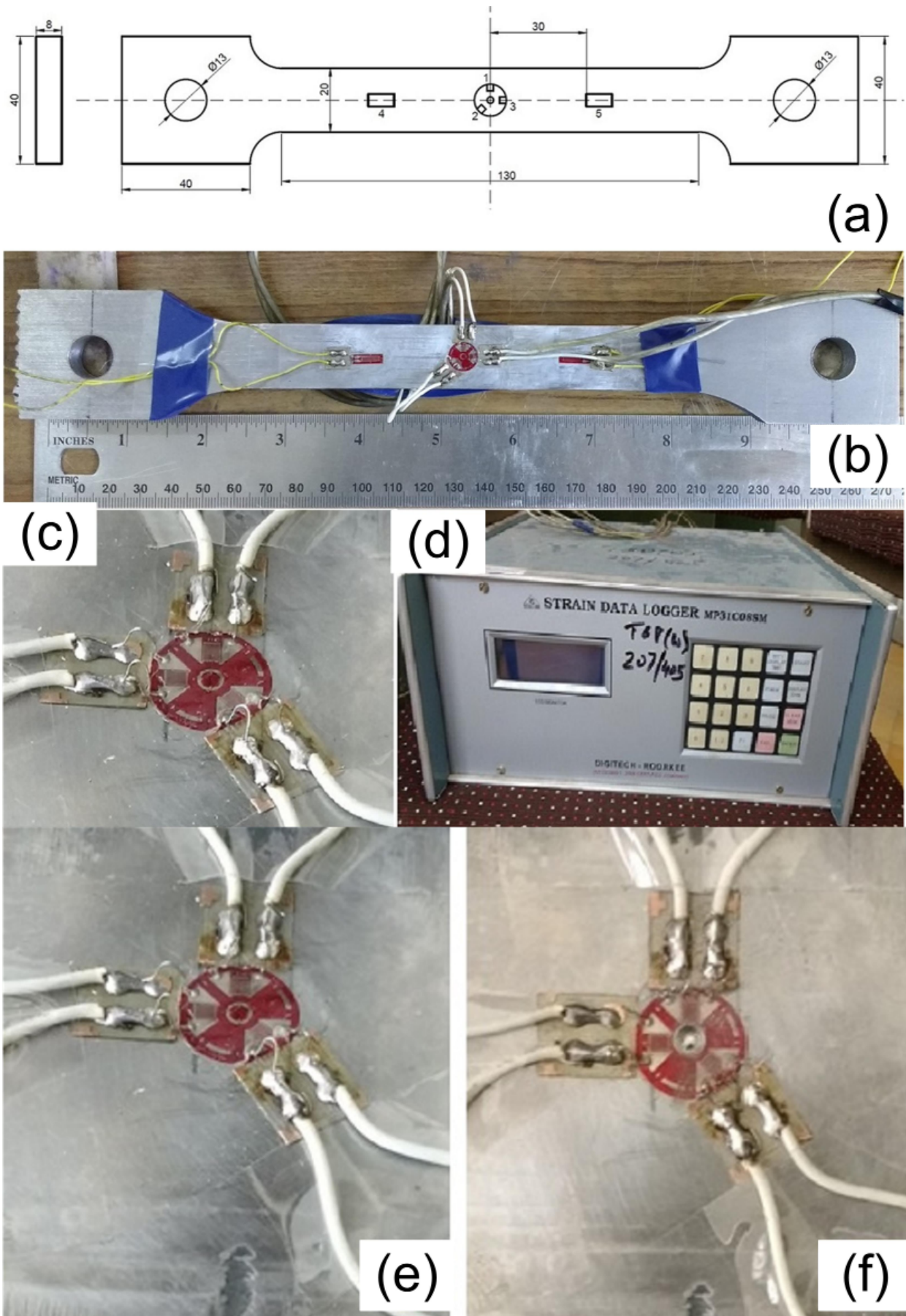
Fig. 1. Tensile specimen for plasticity test and error measurement (a) schematic (1, 2 and 3: strain gauge rosette elements, 4 and 5: single element strain gauge), (b) specimen with strain gauge rosette, (c) Three element strain gauge rosette after pasting and making terminal, (d) strain data logger; Pasted strain rosette over weld fusion zone of TIG (e) before drilling (f) after drilling condition
