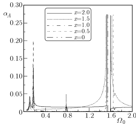
Fig. 4. Displacement amplitudes versus \Omega_0
