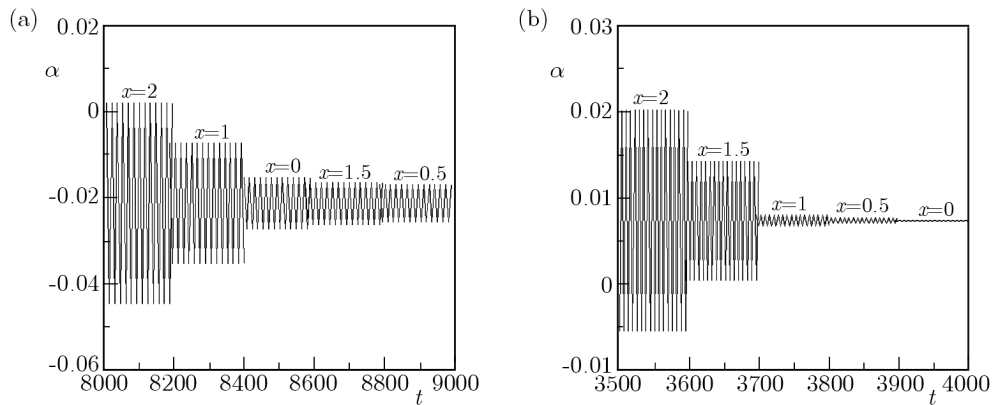
Fig. 3. Angular displacements in the steady state and with \Omega_0 = 0.2 (a) and with \Omega_0 = 0.5 (b)
