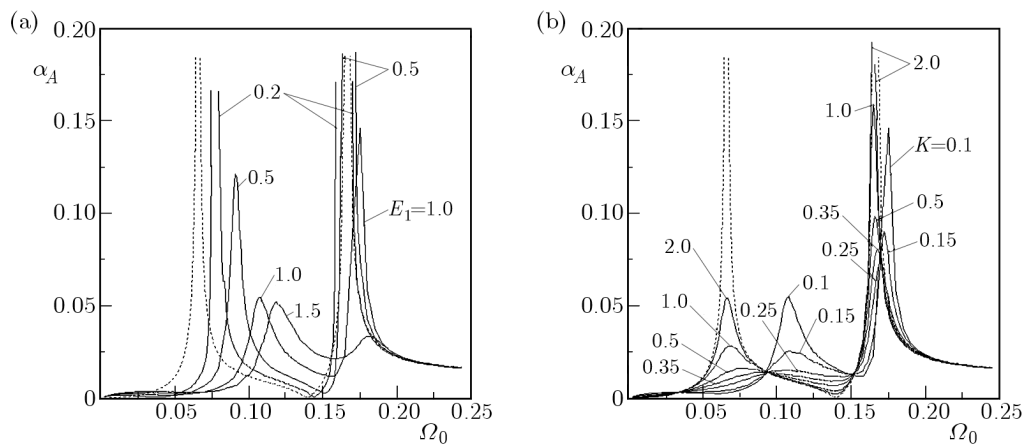
Fig. 5. (a) Effect of E_1 in x = 2 with K = 0.1 ; (b) effect of K in x = 2 with E_1 = 1.0
