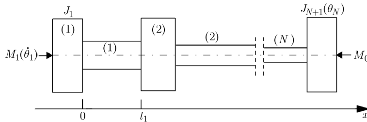
Fig. 1. Discrete-continuous multi-mass torsional system
