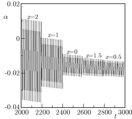
Fig. 2. Angular displacements in the transient state with \Omega_0 = 0.2
