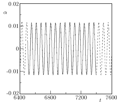
Fig. 6. Comparison of numerical (dashed line) and analytical solutions (continuous line) for displacements of the three-mass system in x = 2 in a steady state with boundary condition (3.3) and \Omega_0 = 0.05
