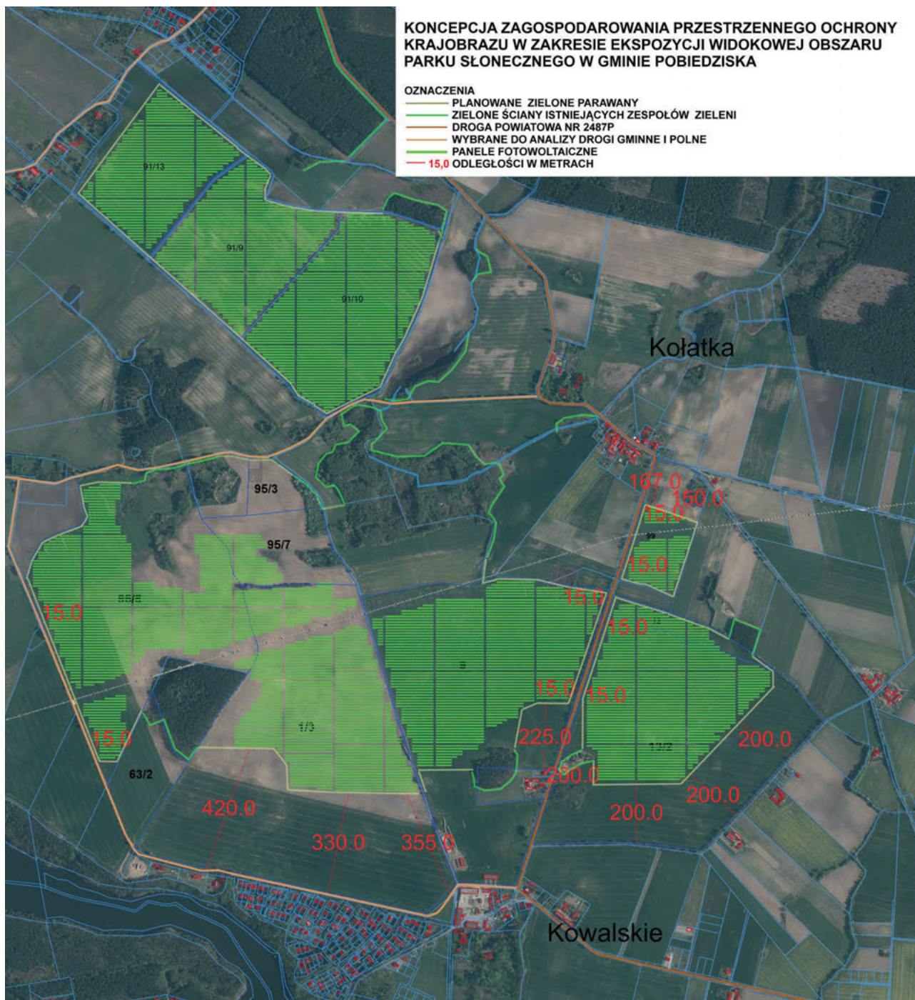
Ill. 3. Plan of the proposal of zoning landscape management in the area of the viewing exhibition of the Pobjedziska Solar Park with marked locations of the 'green screens' and the protection distances of the project site from the main elements of the local landscape. By the authors, 2021.
