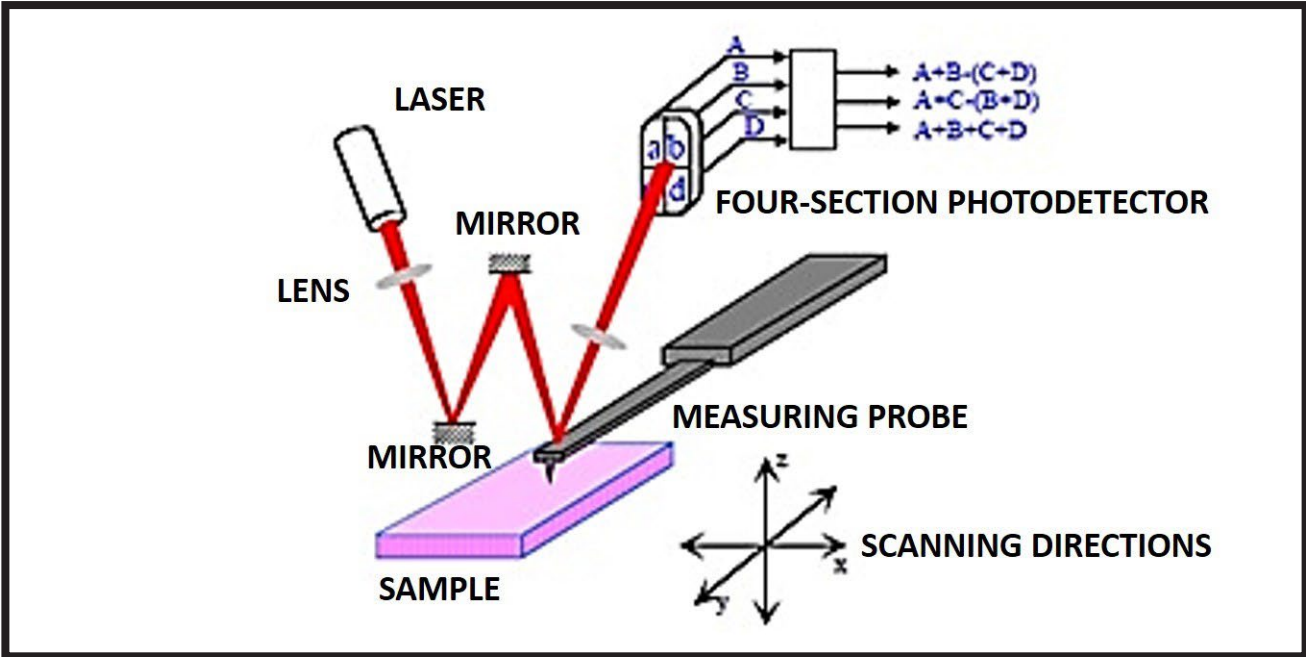
FIG. 5. Scheme illustrating the operating principle of the atomic force scanner [6].
