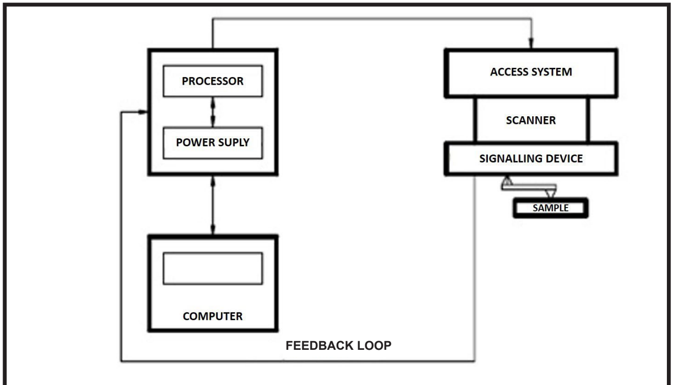
FIG. 4. Block diagram of the atomic force microscope [6].
