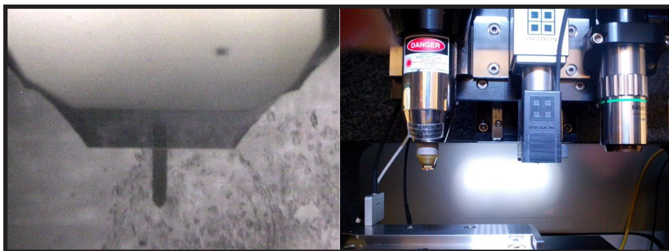
FIG. 3. View of the AFM Q-WM190 probe and measurement heads (AFM, nanoindentation, light microscope) included in the HYSITRON TI950 TriboIndenter.
