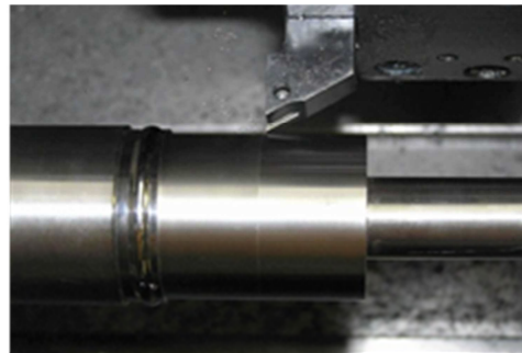
Fig. 6. Finishing with cylindrical plate
