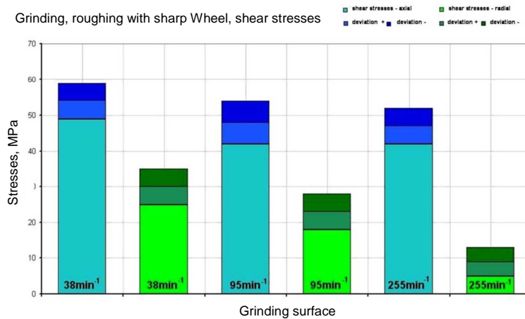
Fig. 21. Diagram of shear stresses in grinding finishing with a sharp wheel
