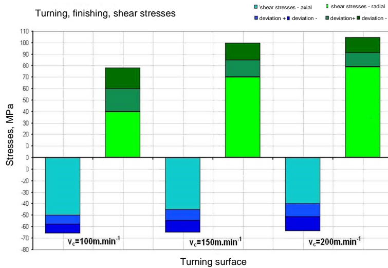
Fig. 13. Diagram of shear stresses in turning finishing
