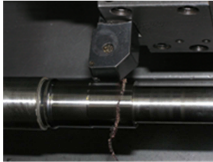
Fig. 4. Roughing with a circular plate of KNB
