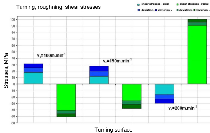
Fig. 11. Diagram of shear stress in rough turning
