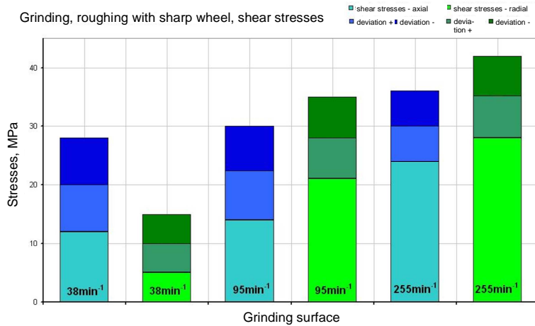
Fig. 19. Diagram of shear stresses in roughing grinding with a very blunt wheel
