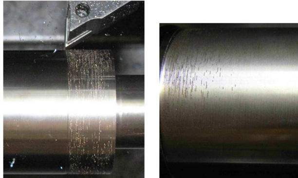
Fig. 22. Poor surface quality due to high wear of cutting plates
