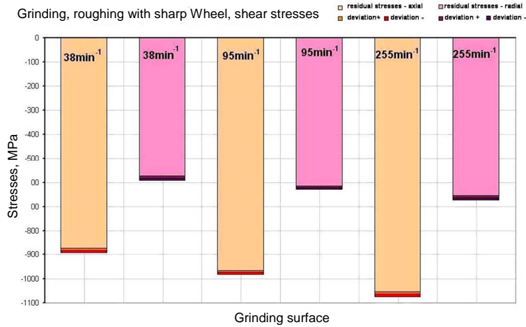
Fig. 20. Diagram of residual stresses in grinding finishing with a sharp wheel
