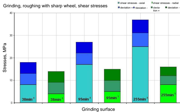
Fig. 17. Diagram of shear stresses in roughing grinding with a bunt wheel
