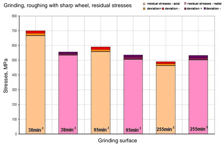
Fig. 18. Graph of residual stresses in grinding of roughing very dull blade
