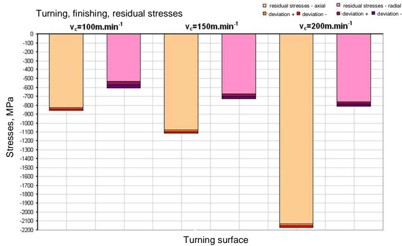
Fig. 12. Diagram of residual stresses in turning finishing
