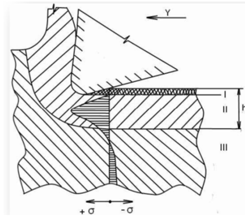
Fig. 1. Diagram of residual stresses in the surface layer under the influence of plastic deformation [1]. I – area of compressive stress induced by friction wedge cutting back on work surface, II – the area of tensile strain introduced by pressing the plastic material, III – unaffected area, such as voltage compensation, I and II
