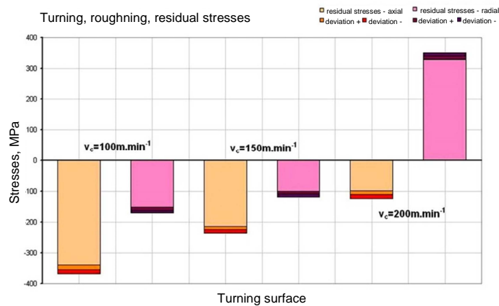
Fig. 10. Diagram of residual stresses in rough turning
