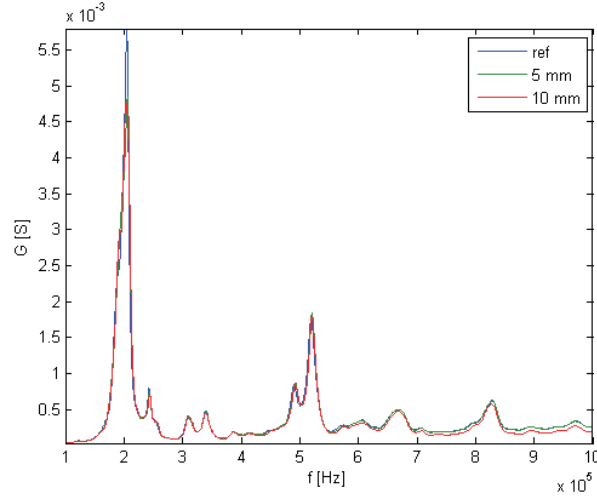
Figure 12: Conductance spectra for the three considered cases.
