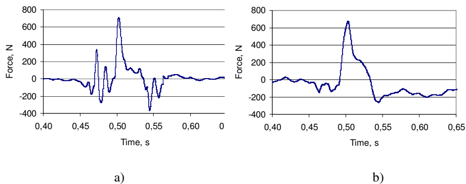
Fig. 6. Dependences of recoil force on time for machine gun 7.62 mm FN MAG: a) real shot, b) simulation
