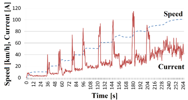
Fig. 2. Speed and motor current registered during chassis dynamometer test
