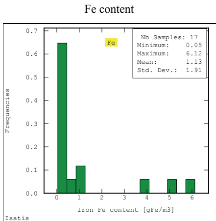
Fig. 15. Distribution histogram of Fe content [g Fe/m 3 ] in underground water in Kłodzko water intake area
