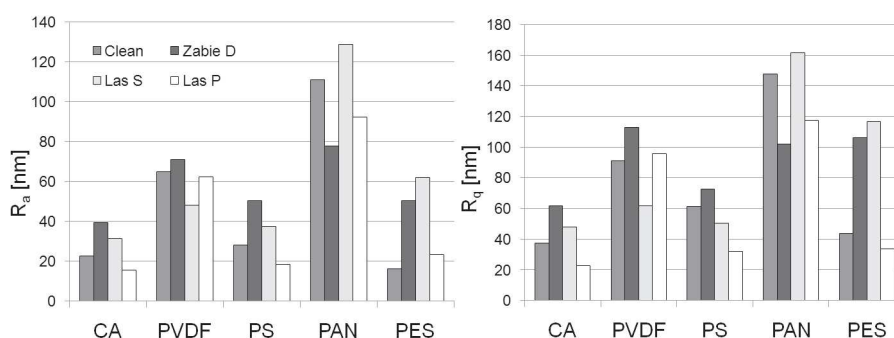
Fig. 2. R_a and R_q of new and used membranes sector 50 \times 50 \mu\text{m}
