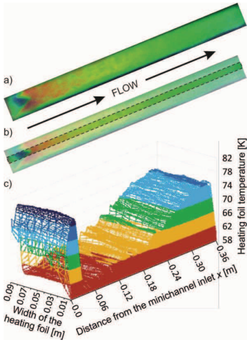
Fig. 10. Liquid crystal image, setting #5 (a); marked area for analysis of temperature distribution (b); two-dimensional temperature distribution of the heating foil (c).
