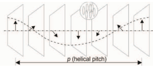
Fig. 2. Simplified diagram of the structure of chiral nematic liquid crystals.
