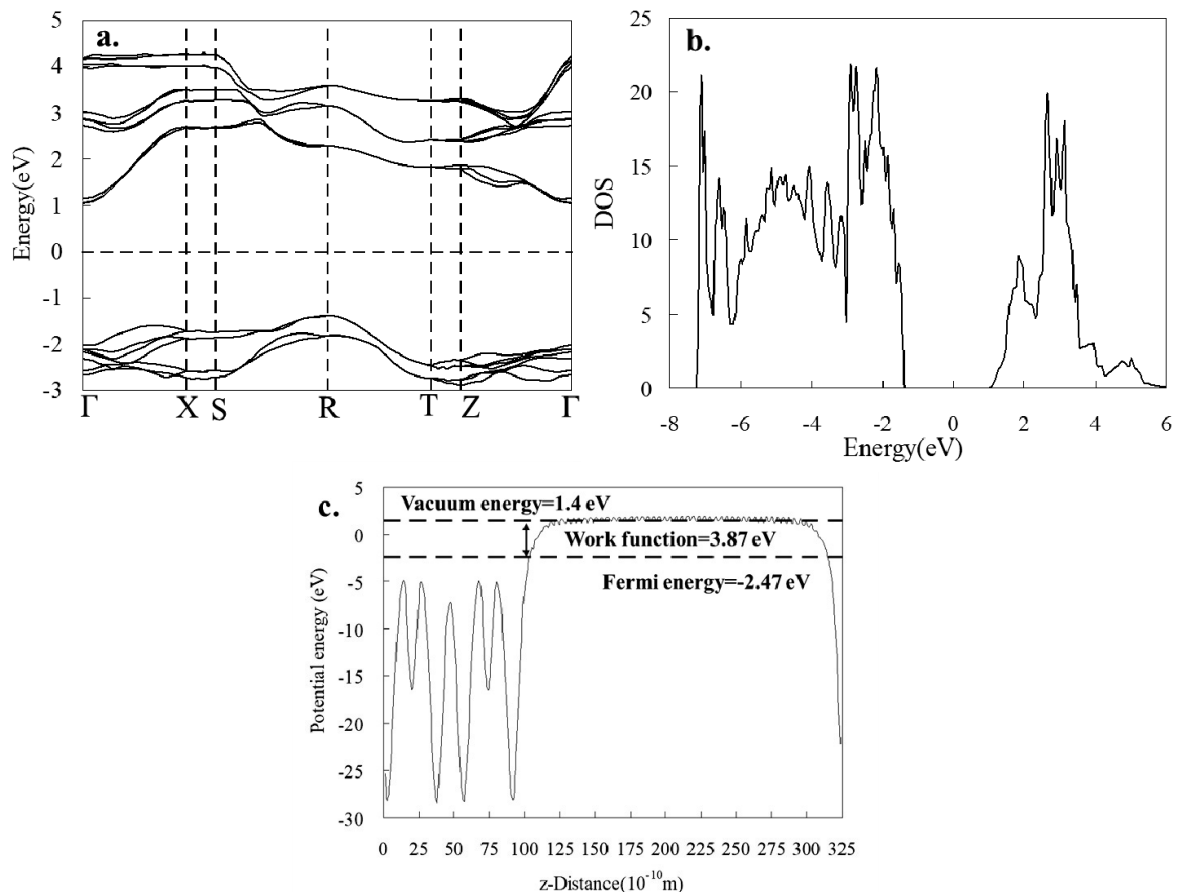
Fig. 14. The band structure (a), DOS (b) and work function (c) of MoO 3 catalyst gained from DFT calculation
