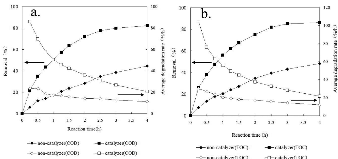
Fig. 11. Effect of reaction time on COD and TOC removal (reaction temperature: 175°C; catalyst dosage: 2.0 g/L)
