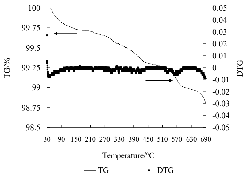
Fig. 7. Thermo-gravimetric analysis results of catalyst ( \text{N}_2 condition)
