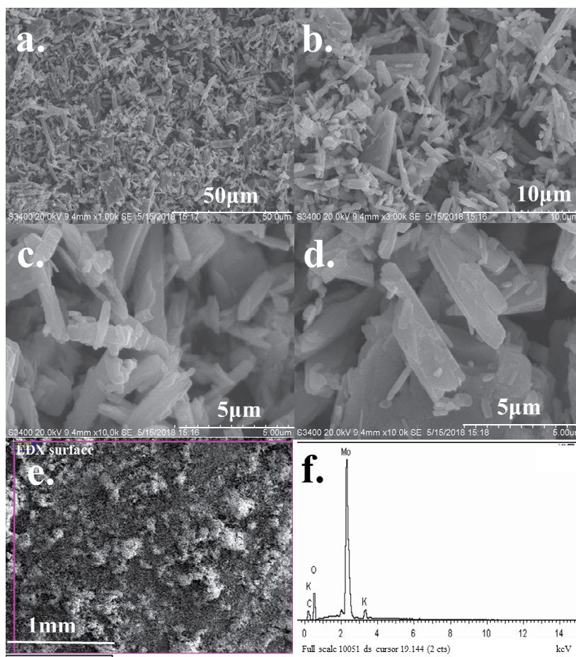
Fig. 5. SEM-EDS analysis results of catalyst
