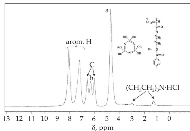
Fig. 2. ^1\text{H} NMR spectrum of PN-acry
