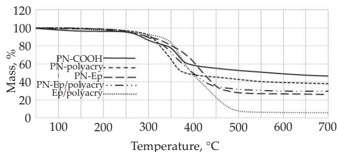
Fig. 12. Stack plot of TG curves of PN-COOH, PN-polyacry, PN-Ep and PN-Ep/polyacry
