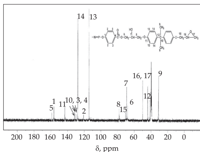
Fig. 7. ^{13}\text{C NMR} spectrum of PN-Ep
