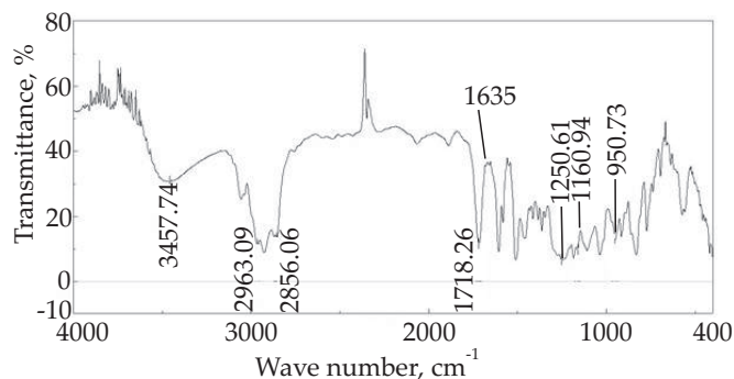
Fig. 10. FT-IR spectrum of PN-Ep/polyacry
