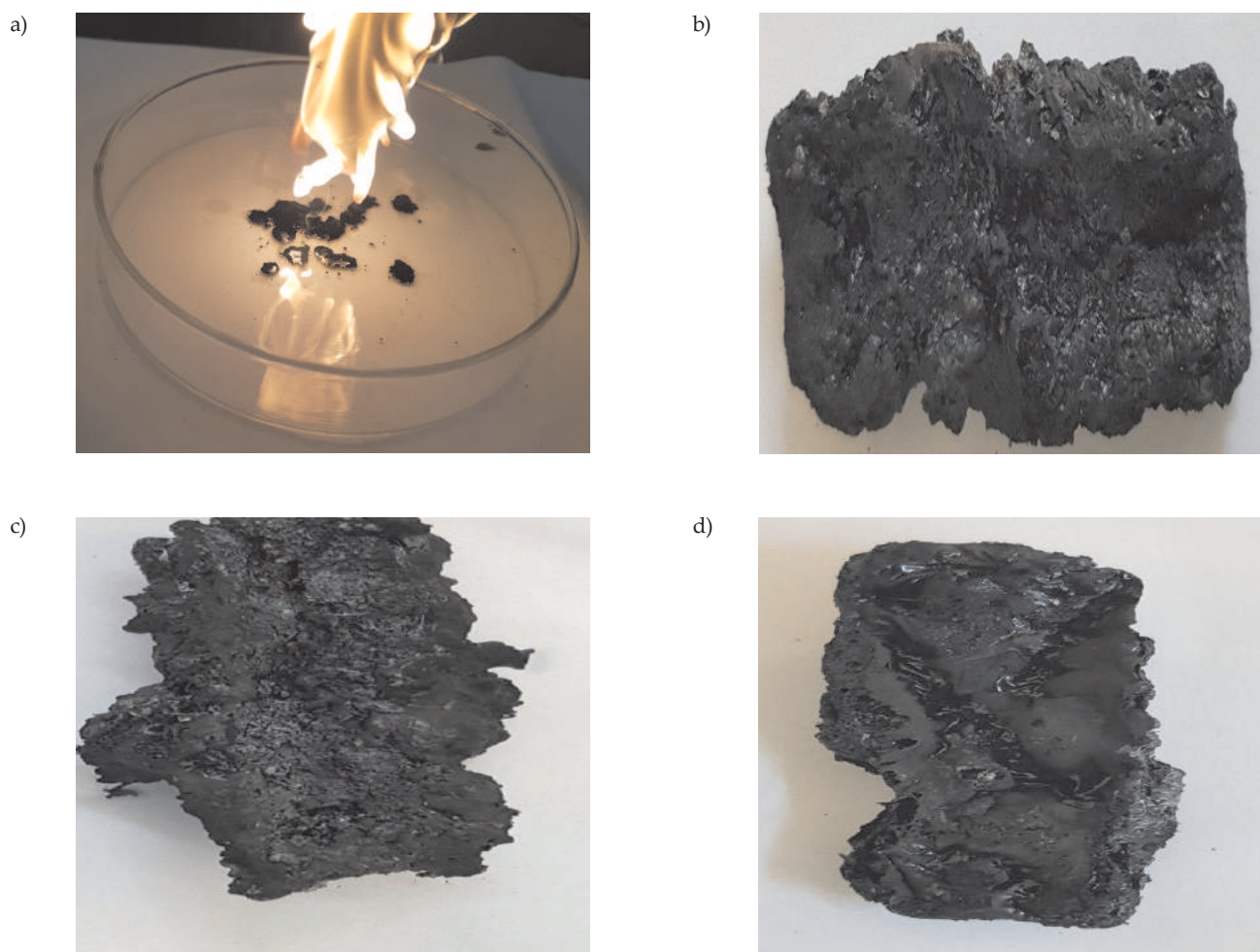
Fig. 13. Digital photos of the: a) burning of cross-linked epoxy resin at atmospheric conditions, b) char residue of PN-polyacry after burning at LOI = 30.5 vol %, c) char residue of PN-Ep after burning at LOI = 27.2 vol %, d) char residue of PN-Ep/polyacry after burning at LOI = 28.0 vol %
