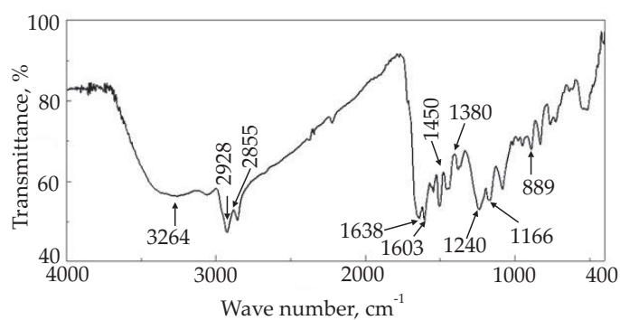
Fig. 15. FT-IR spectrum of the char residue obtained from burning of PN-Ep/polyacry
