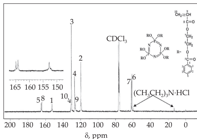
Fig. 3. ^{13}\text{C} NMR spectrum of PN-acry
