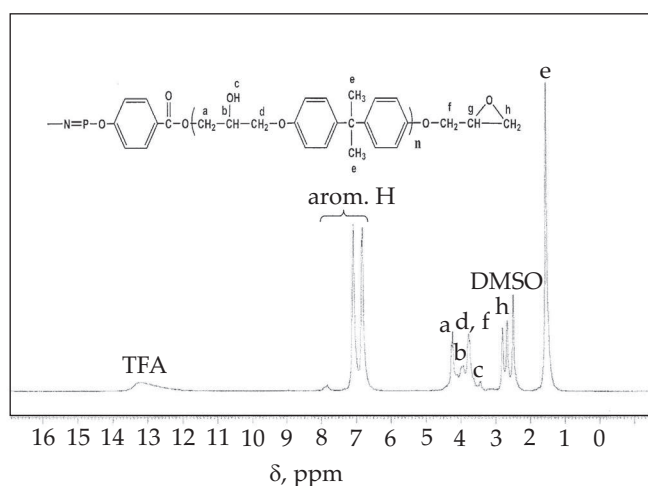
Fig. 6. ^1\text{H NMR} spectrum of PN-Ep
