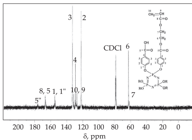
Fig. 9. ^{13}\text{C NMR} spectrum of PN-COOH/acry
