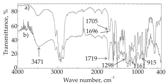
Fig. 5. Stack plot of the FT-IR spectra of reaction of: a) uncatalyzed, b) catalyzed, PN-COOH with epoxy resin
