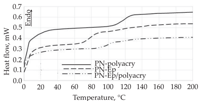
Fig. 11. Stack plot of the DSC thermograms of PN-polyacry, PN-Ep and PN-Ep/polyacry
