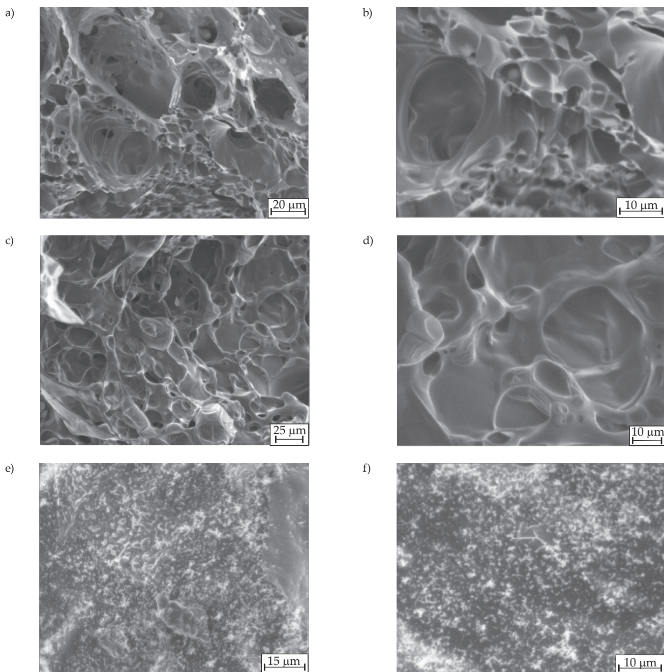
Fig. 14. SEM photomicrographs of the residual char obtained after burning determined LOI of: a), b) PN-polyacry, c), d) PN-Ep/polyacry, e), f) PN-Ep
