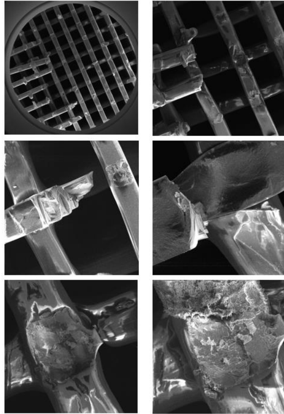
Figure 13 Microscopic observations of samples after 6-month exposure to Ringer's solution – SEM: a) mag.75x, b) mag. 100x, c) mag. 150x, d) mag. 250x, e) mag. 250x, f) mag. 300x
