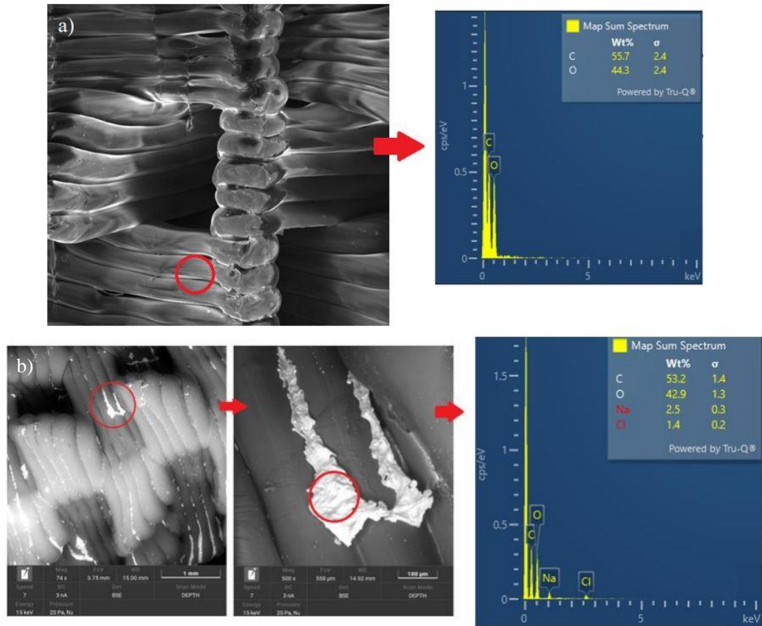
Figure 14 Basic microanalysis of implant chemical elements a) in the initial state, b) after six months of exposure to Ringer's solution
