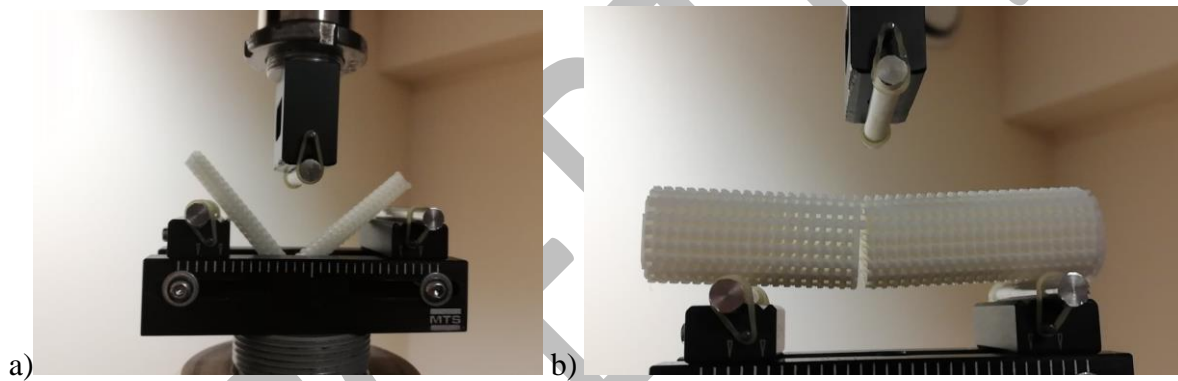
Figure 8 Samples after static three-point bending test: a) group VI, b) group VIII
