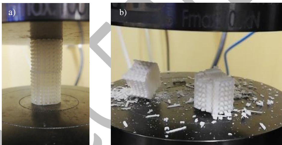
Figure 5 Samples for static uniaxial compression test in the longitudinal direction: a) initial condition (IS), b) after 6 months of exposure to Ringer's solution (R_6)
