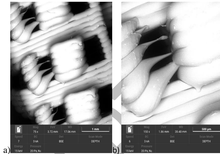
Figure 12 SEM observation of print paths in the initial state a) mag. 75x, b) mag. 150x
