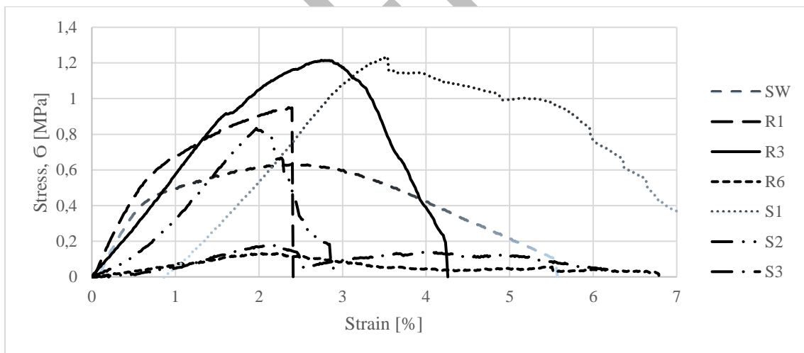
Figure 6 Static uniaxial compression test in the transverse direction: stress-strain relationship for samples with dimensions of 12x24 mm
