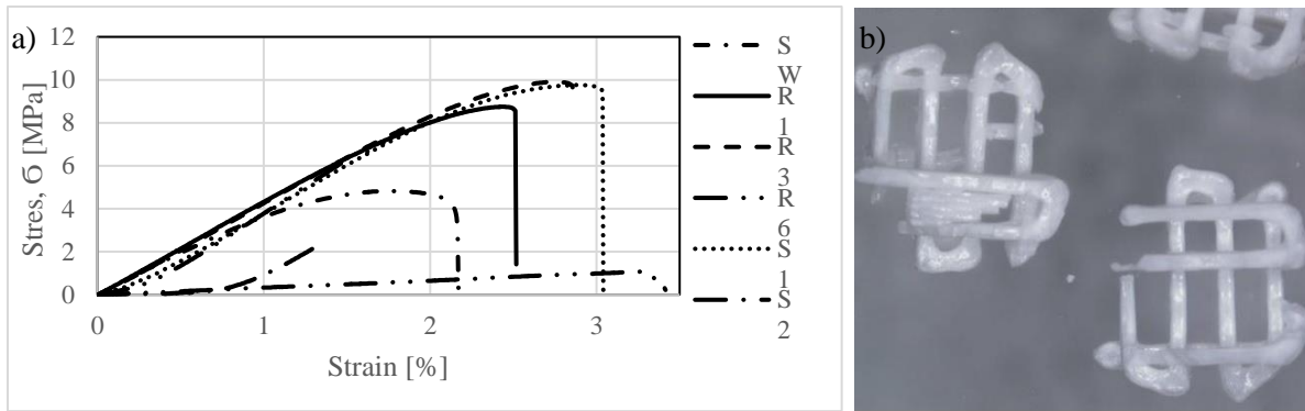
Figure 4 Results of static uniaxial compression test in the longitudinal direction: stress-strain relationship for samples with dimensions of 18x36 mm, b) implants damaged as a result of degradation (group I)
