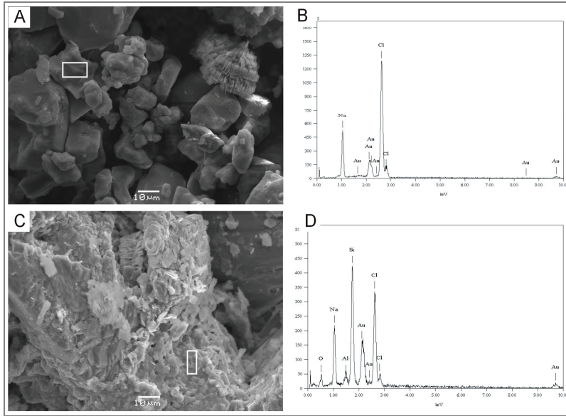
Fig. 6. The sample of sandstones from Żerkowice after completing the test of resistance to the action of de-icing salt: (a) SEM images of the surface of the sample, (b) energy dispersive spectrum (EDS) of halite, (c) SEM images of the interior of the sample, (d) energy dispersive spectrum (EDS) of halite
