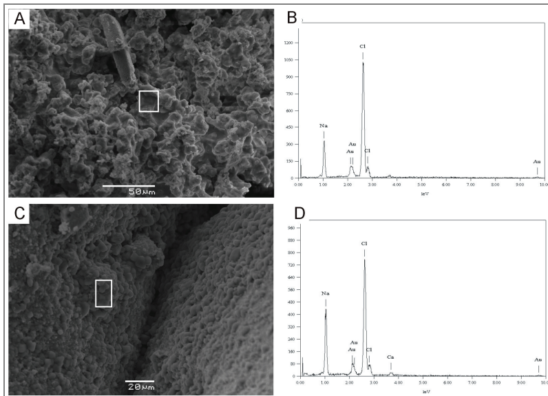
Fig. 7. The sample of limestones from Józefów after completing the test of resistance to the action of de-icing salt: (a) SEM images of the surface of the sample, (b) energy dispersive spectrum (EDS) of halite, (c) SEM images of the interior of the sample, (d) energy dispersive spectrum (EDS) of halite
