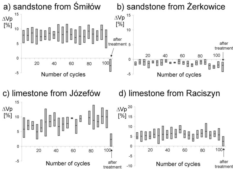
Fig. 10. Changes of the longitudinal wave velocity during the test
