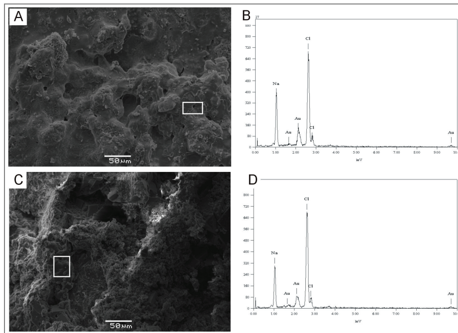
Fig. 8. The sample of limestones from Raciszyn after completing the test of resistance to the action of de-icing salt: (a) SEM images of the surface of the sample, (b) energy dispersive spectrum (EDS) of halite, (c) SEM images of the interior of the sample, (d) energy dispersive spectrum (EDS) of halite
