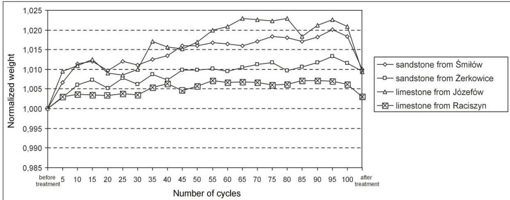
Fig. 9. Weight evolution during subsequent test cycles
