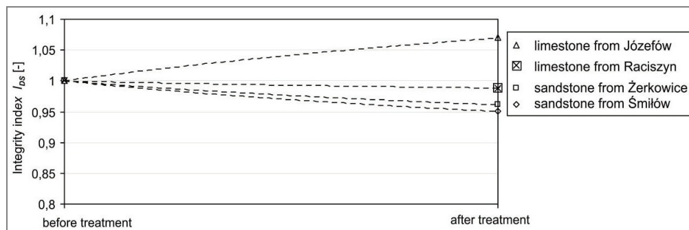
Fig. 11. Average values of the integrity index after the action of the de-icing salt
