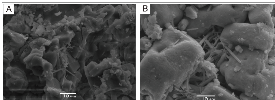
Fig. 4. SEM images of the surface of the sample after completing the test of resistance to the action of de-icing salt: (a) elongated gypsum crystals in the pore space of limestone from Józefów, (b) elongated gypsum crystals in the pore space of sandstone from Żerkowice
