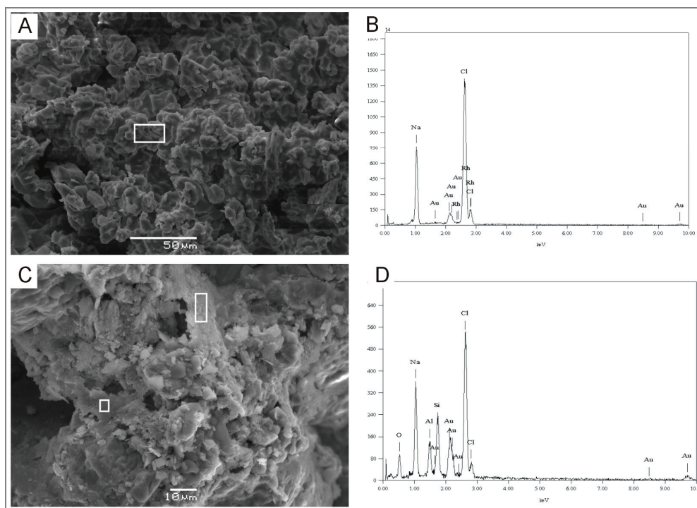
Fig. 5. The sample of sandstones from Śmiałów after completing the test of resistance to the action of de-icing salt: (a) SEM images of the surface of the sample, (b) energy dispersive spectrum (EDS) of halite, (c) SEM images of the interior of the sample, (d) energy dispersive spectrum (EDS) of halite
