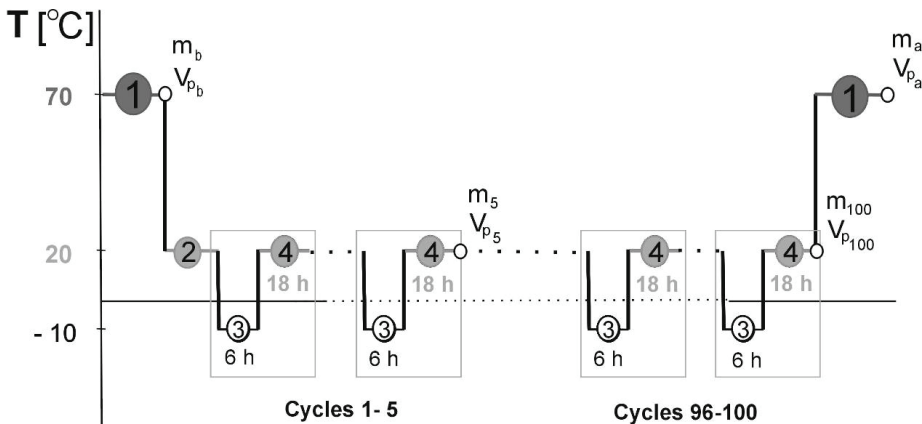
Fig. 2. Diagram of the study: 1 – drying to a constant weight, 2 – saturation with a 10% solution of the de-icing salt to a constant weight, 3 – the action of negative temperatures, 4 – immersion in a 10% solution of the de-icing salt
