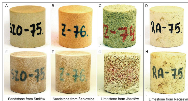
Fig. 3. The appearance of the samples after completing the test of resistance to the action of the de-icing salt: (a)–(d) the reference samples (before the test); (e)–(h) the samples after the test
