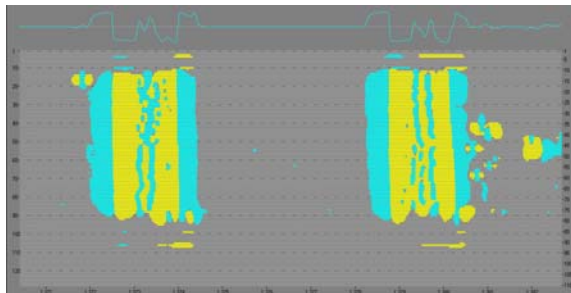
Fig. 6. 2D view of a splice in Belt Analysis software
