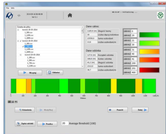
Fig. 8. Visualization of test results using Diagbelt system
