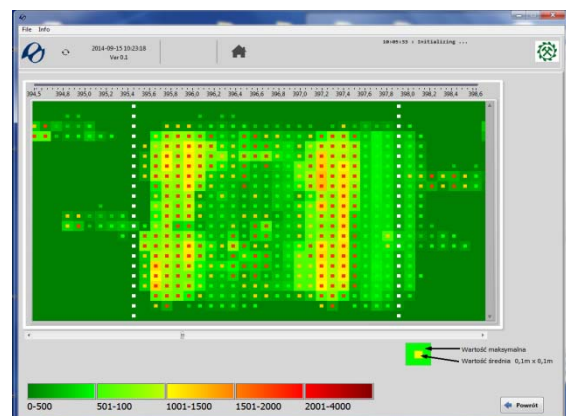
Fig. 9. Image of properly performed splice in the window of Diagbelt software
