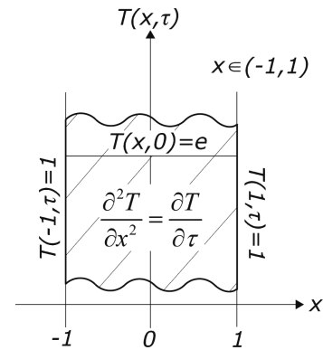
Fig. 1. Initial boundary value problem
