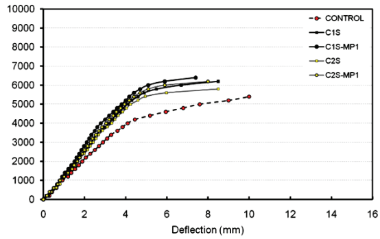
Fig. 13. Effect of using plastic mesh MP1 compared to control beam and strengthening using only concrete layer without meshes
