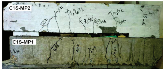
Fig. 20. Crack pattern of samples (from up to down; C1S-MP2 and C1S-MP1)
