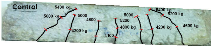
Fig. 18. Crack pattern of control beam samples
