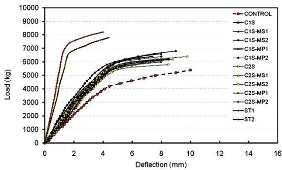
Fig. 17. Load-deflection relationships for all tested beams
