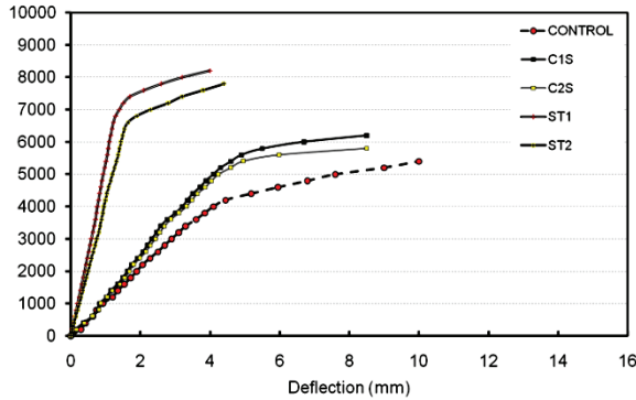
Fig. 10. Effect of using steel plates compared to 2cm thickness C1S and C2S
