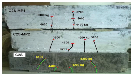
Fig. 22. Crack pattern of samples (from up to down; C2S-MP1, C2S-MP2 and C2S)
