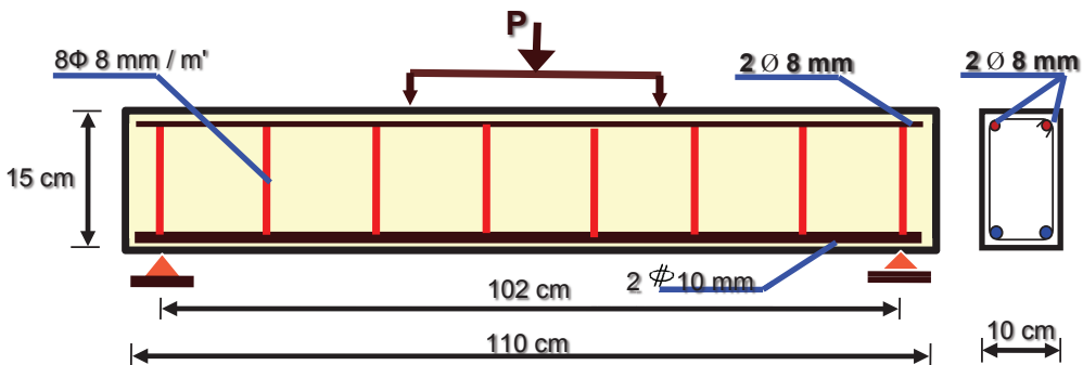
Fig. 1. Detailing of tested beams
