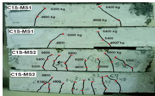
Fig. 19. Crack pattern of samples (from up to down; C1S-MS1, C1S-MS1, C1S-MS2 and C1S-MS2)
