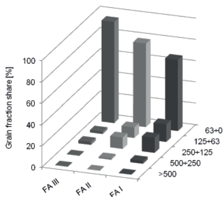
Fig. 2. The share of individual grain fractions for the examined fly ashes.
