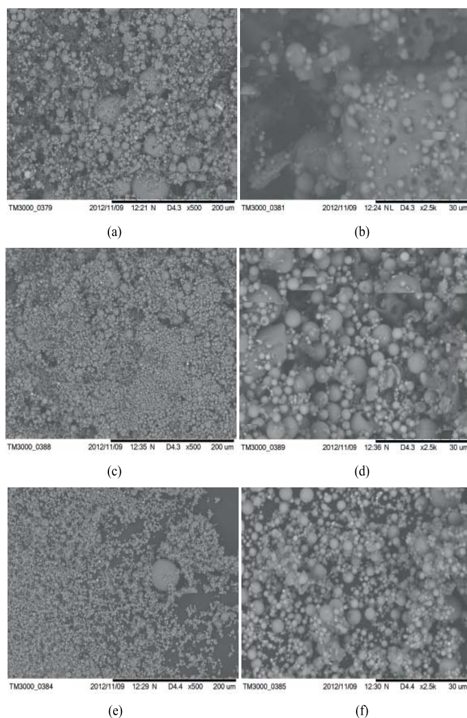
Fig. 1. Images of fly ashes: a, b) FA I ; c, d) FA II ; e, f) FA III zoomed 500x and 2500x.
