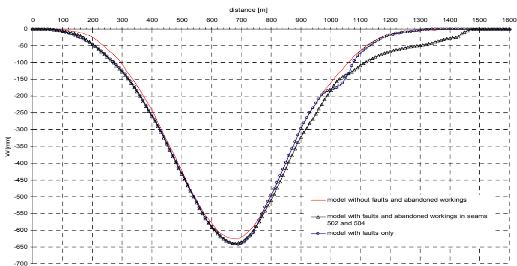
Fig. 5. Subsidence determined on the basis of a numerical model
