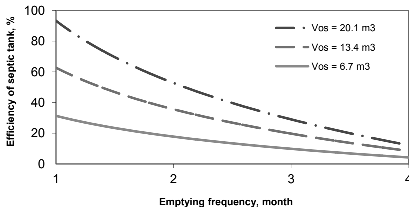
Fig. 11. Efficiency of the septic tank in relation to its emptying frequency
