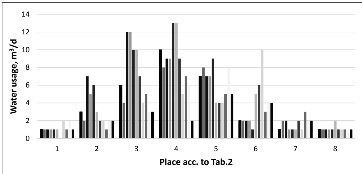
Fig. 6. Water usage in investigated plants in 11 consecutive days of selected weeks
