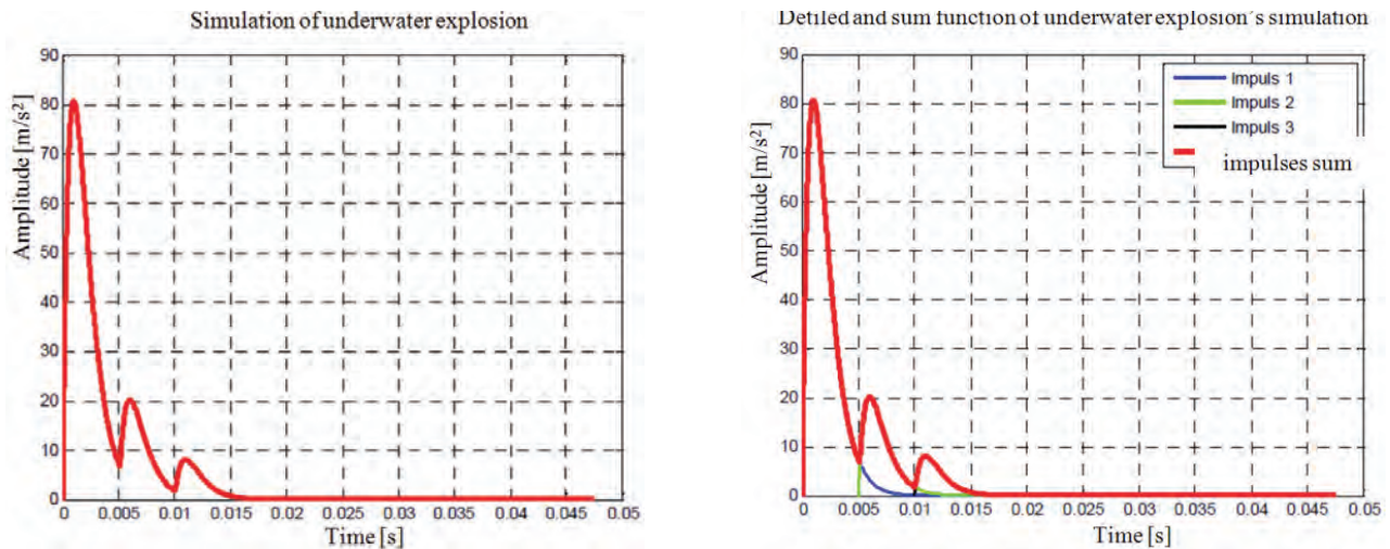
Fig. 1. Simulation of underwater explosion with three gas bubbles and assumed quotient of subsequent amplitude: A1/A2 = 0.25 and A1/A3 = 0.1 [10]
