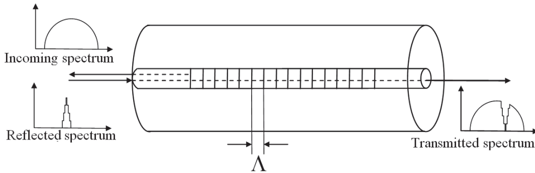
Fig. 2. Scheme of a FBG sensor with reflected and transmitted spectra
