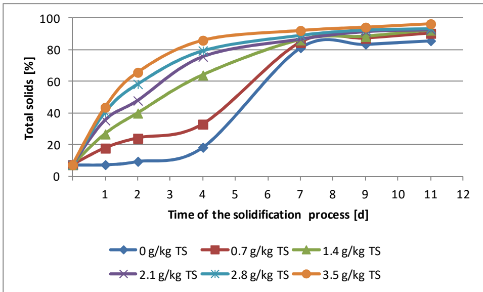
Fig. 2. Changes of the total solids during solidification with cement Gorkal G 40
