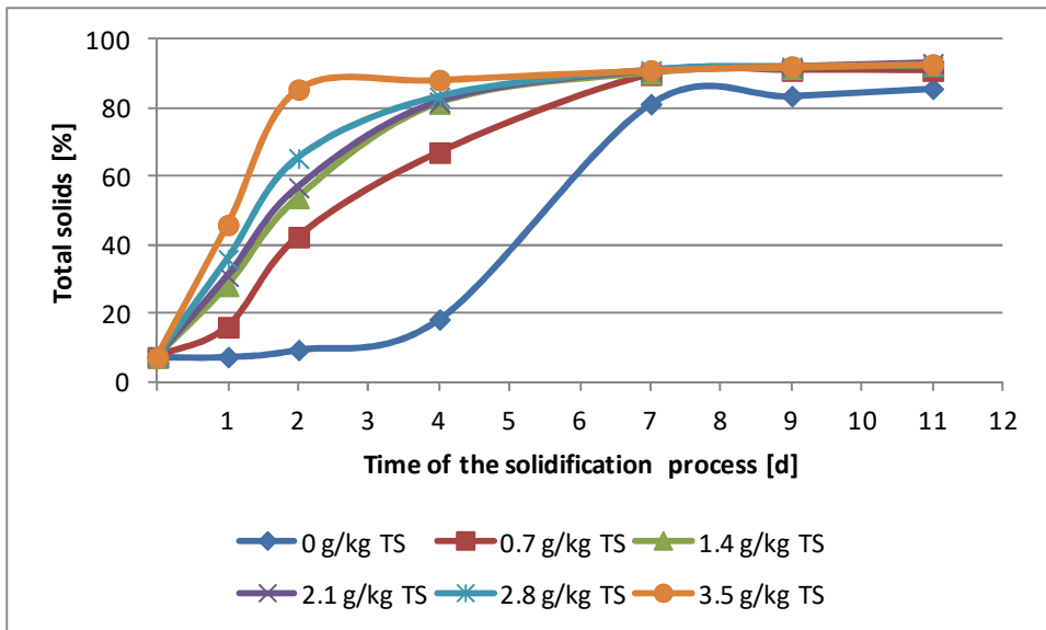
Fig. 3. Changes of the total solids during solidification with cement Gorkal G 50
