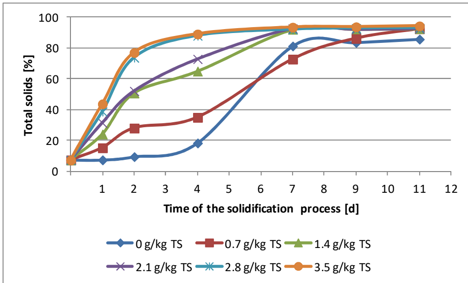
Fig. 4. Changes of the total solids during solidification with cement Gorkal G 70
