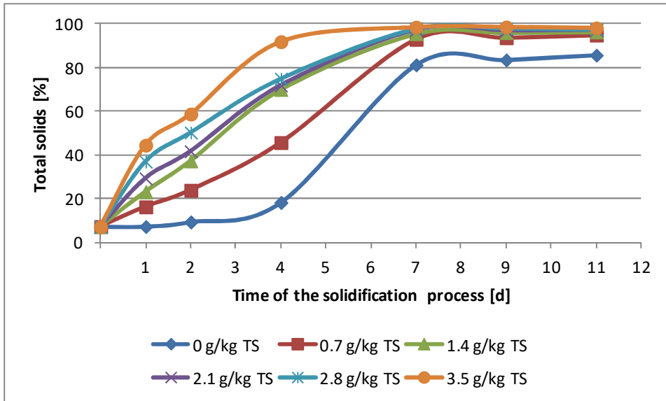
Fig. 1. Changes of the total solids during solidification with CaO
