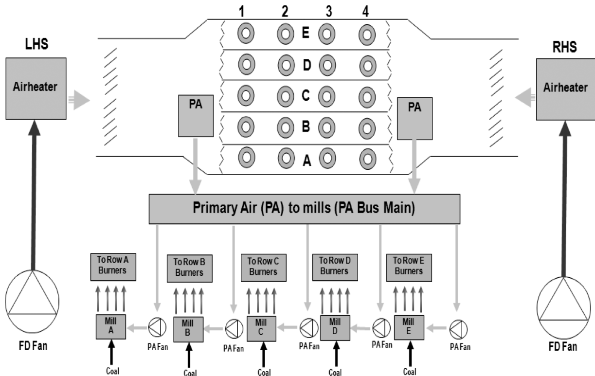
Fig. 7. Wind-box arrangement following RTS modification
