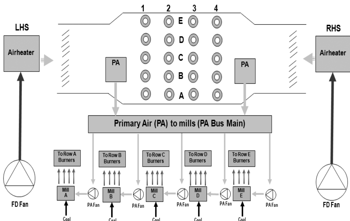
Fig. 6. Wind-box arrangement prior to decommissioning
