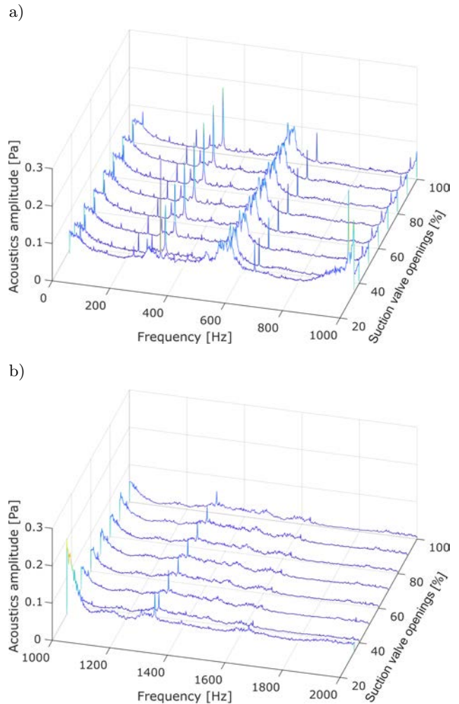
Fig. 7. Acoustic signal in frequency domain under various suction valve opening and the frequency range from (a) 0 Hz–1 kHz to (b) 1–2 kHz at 103 l/min.
