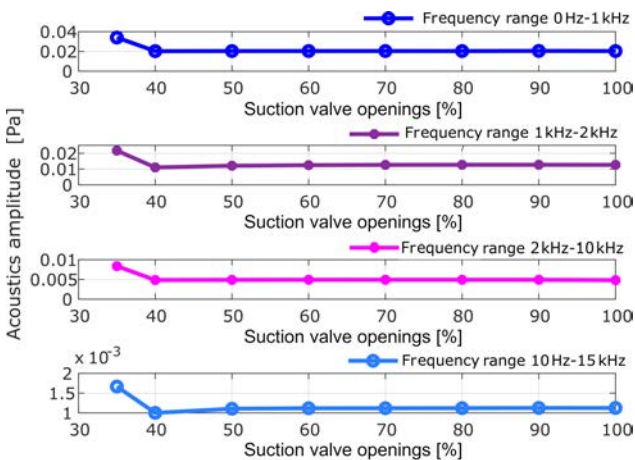
Fig. 8. Mean acoustic amplitude value of the frequency range from 0 Hz to 15 kHz at 103 l/min.
