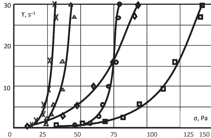
Fig. 2. Shear characteristics of raw material samples in the composition: ○ – apple; Δ – viburnum; × – black chokeberry; ◇ – pumpkin; – beets □
