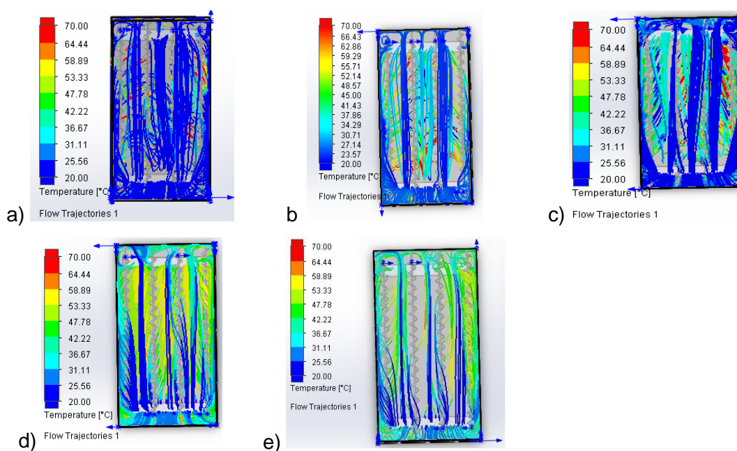
Fig. 5. Distribution of air temperature in the volume of the air channel of the collector depending on its height: a) h = 0.25 m; b) h = 0.2 m; c) h = 0.15 m; d) h = 0.1 m; e) h = 0.08 m.
