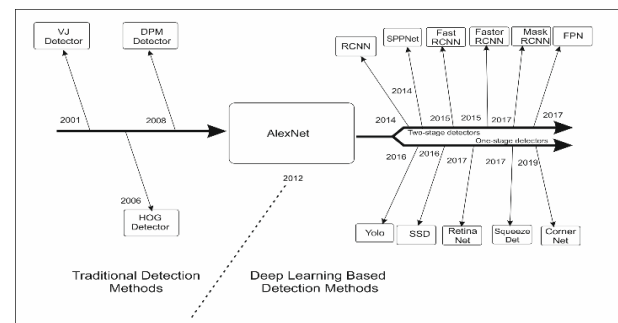
Fig. 4. Object detection milestones [21] [24] DPM, RCNN
