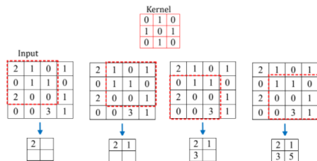
Fig. 5. Convolutional Operation with image matrix (4×4) with kernel matrix (3×3)
