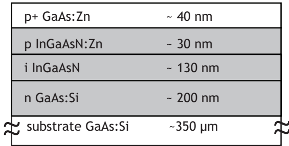
Fig. 1. Scheme of the epitaxial structure of p-i-n InGaAsN solar cell.
