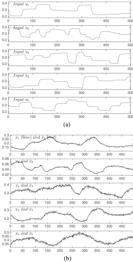
Fig. 4. Test database \mathcal{B}^t : input (a) and output (b).
