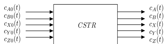
Fig. 1. System structure.
