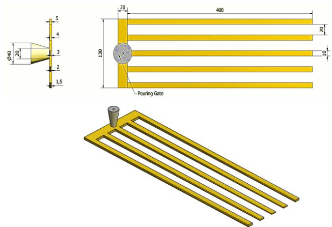
Fig. 3. Mold pattern design
