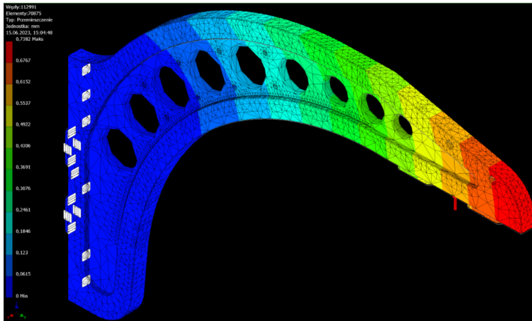
Fig. 6. Simulation result - displacement
