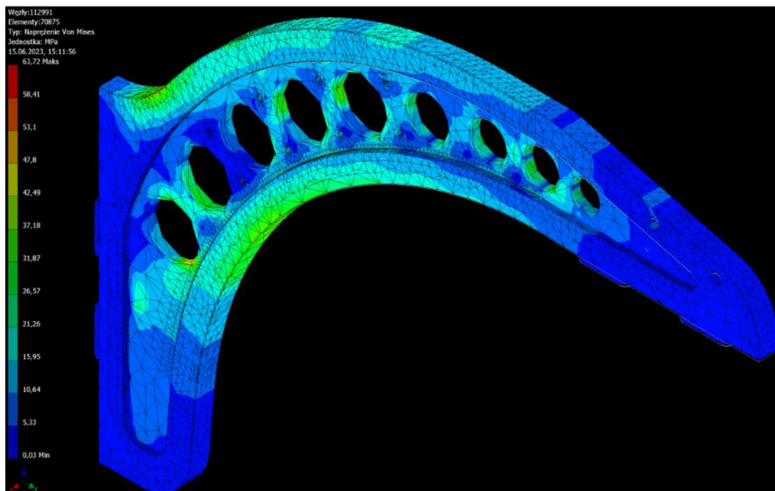
Fig. 7. Simulation result - reduced stress
