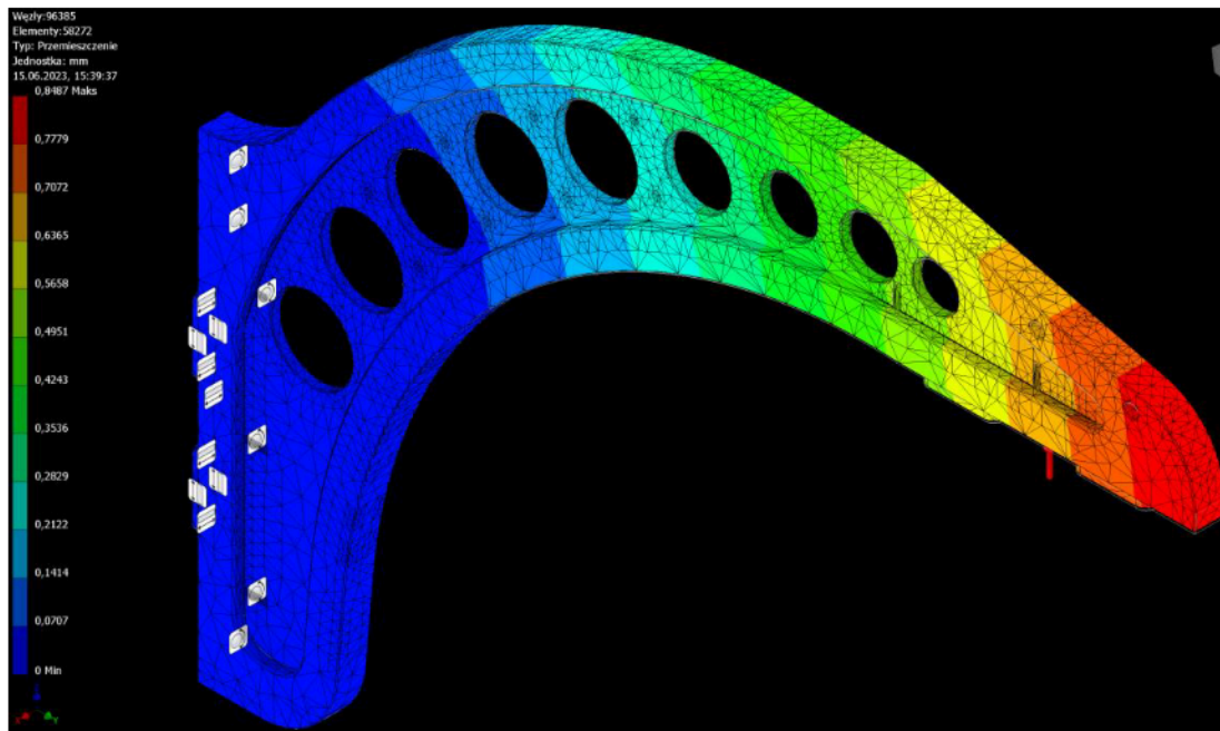
Fig. 9. Result of the simulation - displacement
