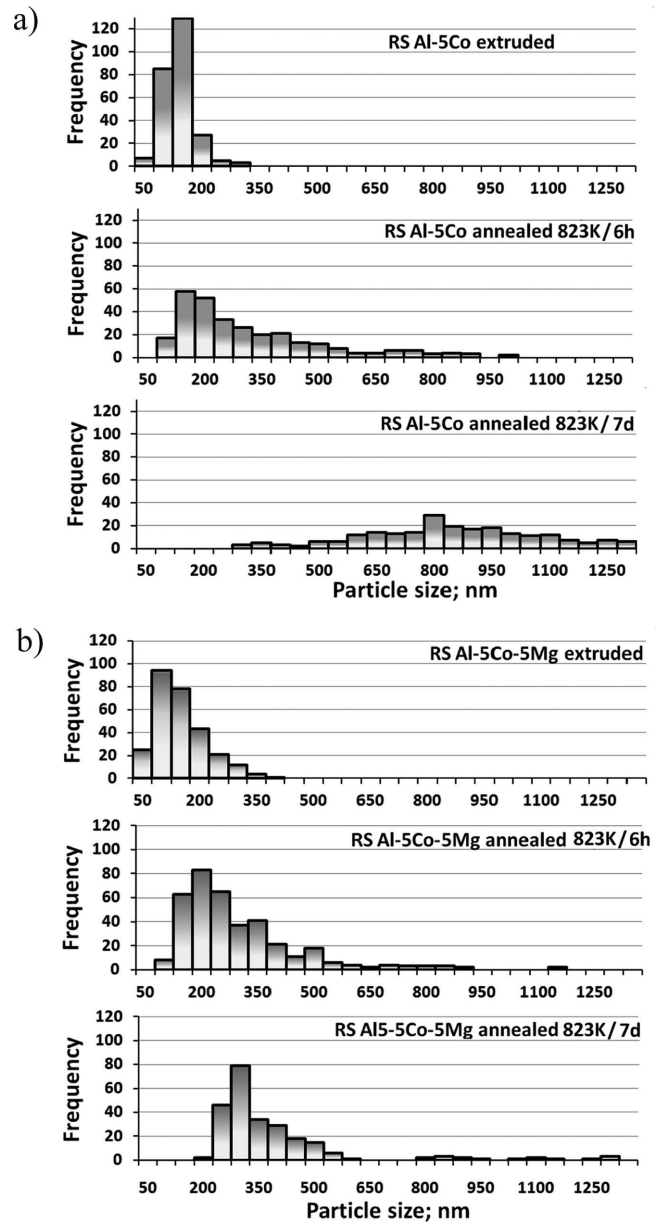
Fig. 10. Distribution of \text{Al}_2\text{O}_3 particles in as-extruded and annealed RS alloys (a) Al-5Co; (b) Al-5Co-5Mg. Heat treatment conditions (823K/6h, 823K/168h) are marked in the figure
