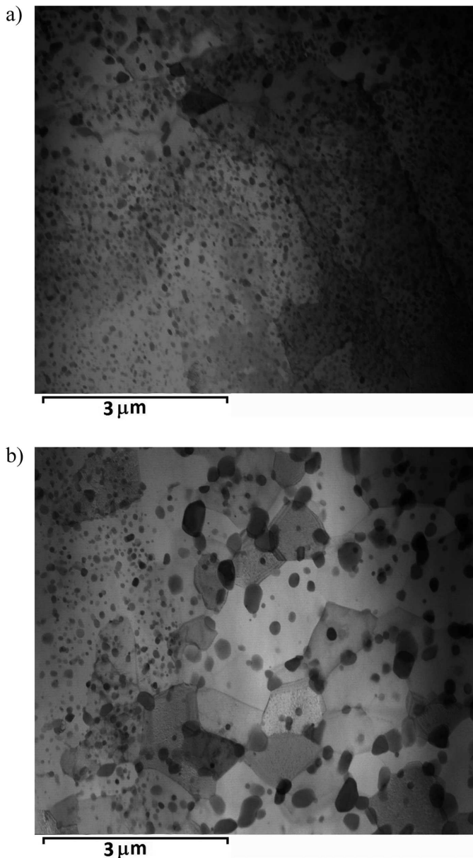
Fig. 11. STEM structure of RS alloys deformed \epsilon_r \cong 0,4 at 773K by compression: (a) Al-5Co (b) Al-5Co-5Mg
