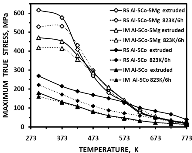
Fig. 2. Effect of deformation temperature on the maximum flow stress for IM Al-5Co, RS Al-5Co, IM Al-5Co-5Mg and RS Al-5Co-5Mg as extruded alloys and samples annealed at 823K/6h. The materials and heat treatment conditions are listed in the legend
