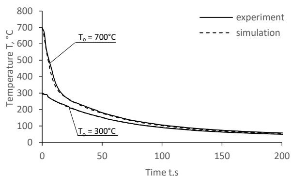
Fig. 7. Comparison of the results of numerical calculations and experimental tests for cooling in oil (22°C) from the initial temperature of 700°C and 300°C
