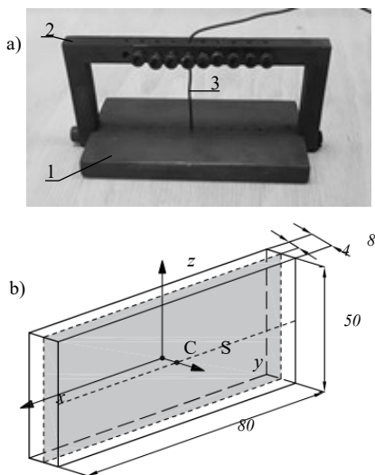
Fig. 2. Test sample a) image of the sample prepared for testing; 1 – sample, 2 – holder, 3 – thermocouple; b) dimensions of the sample of 4 mm in the sample (half of the thickness).
