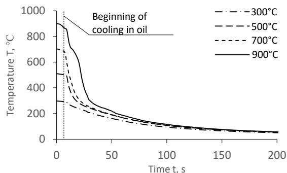
Fig. 3. Temperature changes in the sample core as a function of the cooling time in oil
