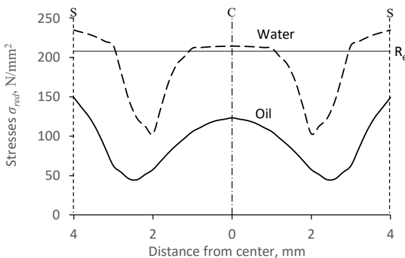
Fig. 12. Distribution of stress \sigma_{red} on the cross-section of the rib after time \Delta t at cooling from 700^\circ\text{C} to 22^\circ\text{C}
