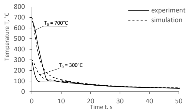
Fig. 8. Comparison of the results of numerical calculations and experimental tests for cooling in water (22°C) from the initial temperature of 700°C and 300°C
