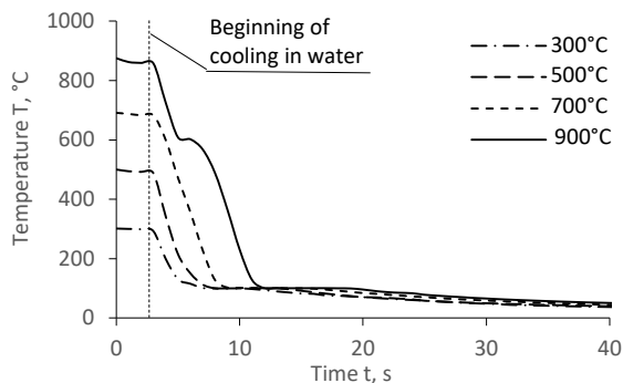
Fig. 4. Temperature changes in the sample core as a function of the cooling time in water
