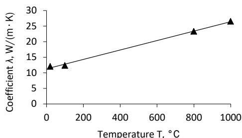
Fig. 5. Thermal conductivity coefficient vs temperature for cast 1.4849
