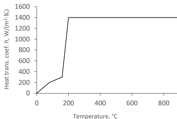
Fig. 6. Heat transfer coefficient vs temperature function adapted for oil
