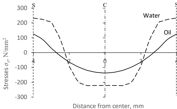
Fig. 11. Distribution of stresses \sigma_x on the cross-section of the rib after time \Delta t at cooling from 700^\circ\text{C} to 22^\circ\text{C}
