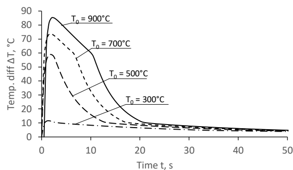
Fig. 9. Difference in temperature between the rib core and surface during cooling in oil
