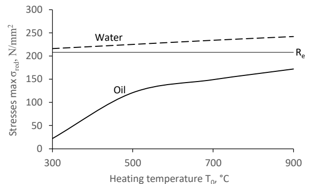
Fig. 13. The maximum reduced stress determined as a function of the initial temperature for cooling in water and oil in 22^\circ\text{C}
