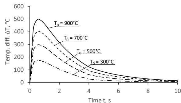
Fig. 10. Difference in temperature between the rib core and surface during cooling in water
