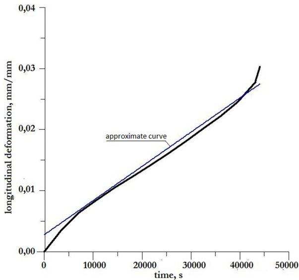
Fig. 3. Approximation of the experimental creep curve using Maxwell's rheological model
