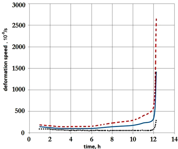
Fig. 2. Graphs of longitudinal creep velocity (dotted line), transverse (solid line) and volume (broken line) representing a dependence of the tested sample on time
