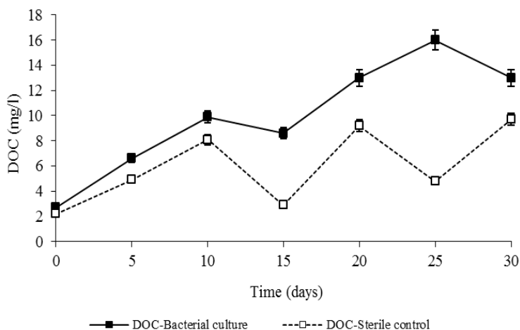
Fig. 2. Organic carbon mobilization from shale organic matter – the changes of the dissolved organic carbon (DOC) concentration in the aqueous phase of bacterial cultures during growth of microorganisms.
