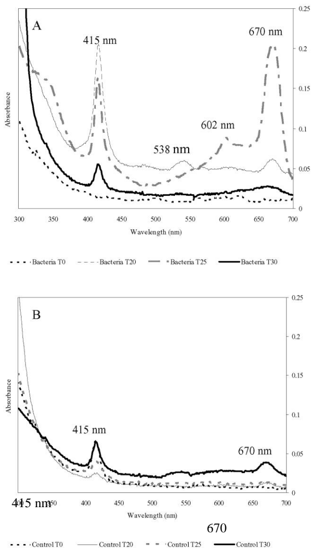
Fig. 4. UV-Vis spectra of chloroform extracts of the aqueous phase of bacterial cultures (A) and sterile control (B) containing organic matter extracted from black shale at the beginning of the experiment (T0), and after 25 (T25) and 30 days (T30) of cultivation
