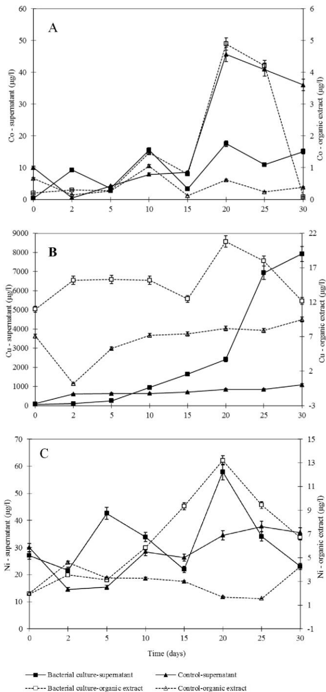
Fig. 3. Concentration of cobalt (A), copper (B) and nickel (C) in the aqueous phase and chloroform extracts of bacterial cultures and sterile controls over the 30 days of cultivation
