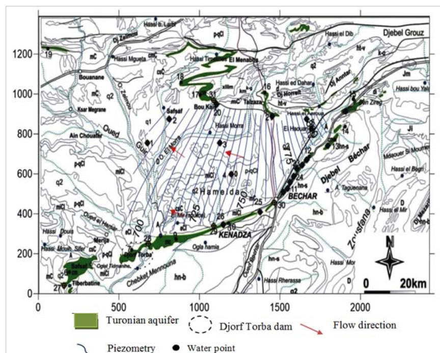
Fig. 3. Piezometric map; own elaboration
