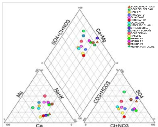
Fig. 4. Triangular diagram Piper companion of Turonian table; source: own study
