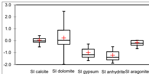
Fig. 5. Box plots illustrating the variation of the saturation indices (SI) of certain minerals of the aquifer formation; source: own study
