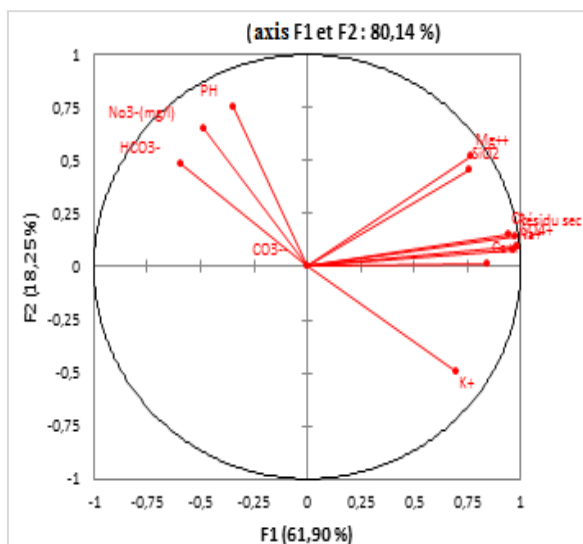
Fig. 6. Graphical representation in principal component analysis (PCA) waters; source: own study
