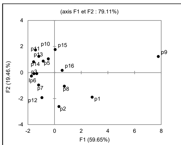
Fig. 7. Graphical representation of individuals; source: own study
