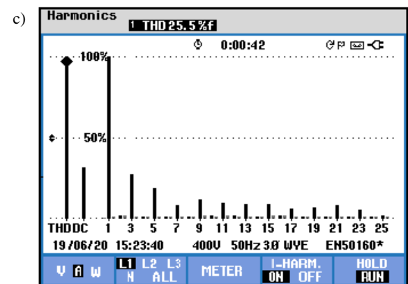
Fig. 12. a) voltage from the utility grid, b) connected load current, c) harmonic distortion results
