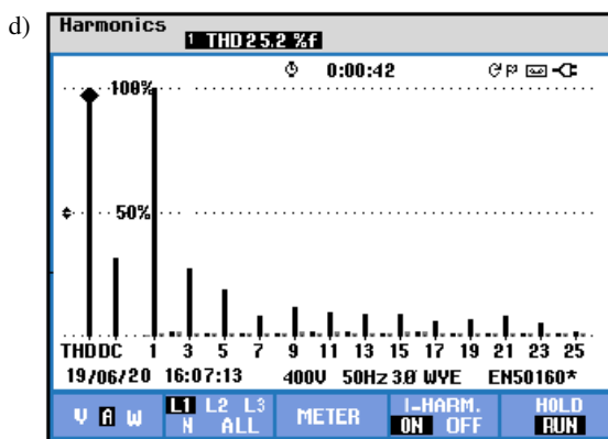
Fig. 9. Results from experiments with balanced voltages and unbalanced loads: a) voltage from the utility grid, b) connected load current, c) connected load current, current of the grid, and compensation current, d) harmonic distortion results
