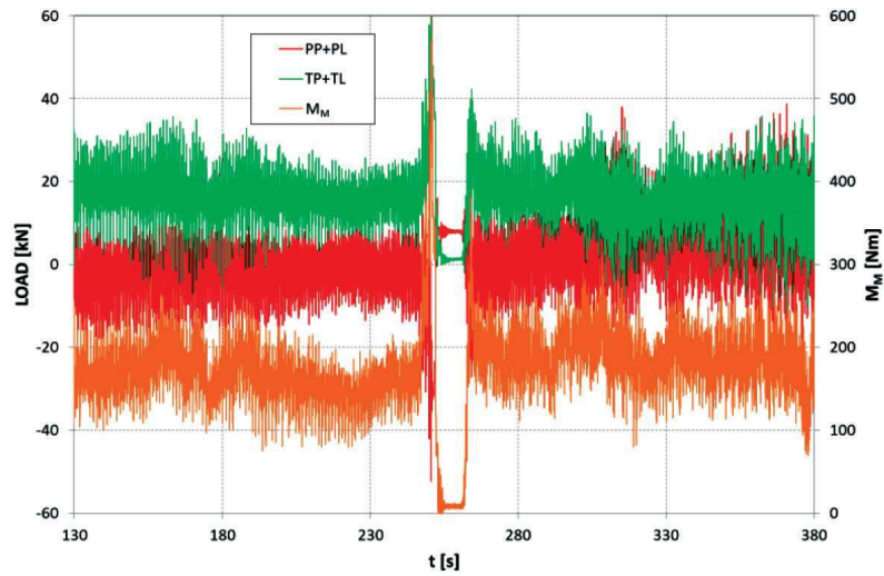
Fig. 7. Time functions of dynamic loads of front (PP+PL) and back supports (TP+TL) resulting from cutting process for upper cut
