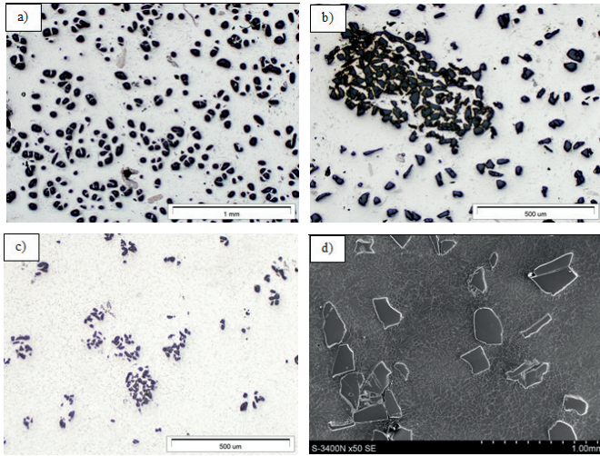
Fig. 3. Reinforcement distribution in different composites; a, b) 45 \mu\text{m} particulates, LM; c) 15 \mu\text{m} particulates, LM; d) 250 \mu\text{m} particulates, SEM
