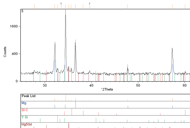
Fig. 8. XRD analysis results for SiC-WE43 composite cast from 780°C
